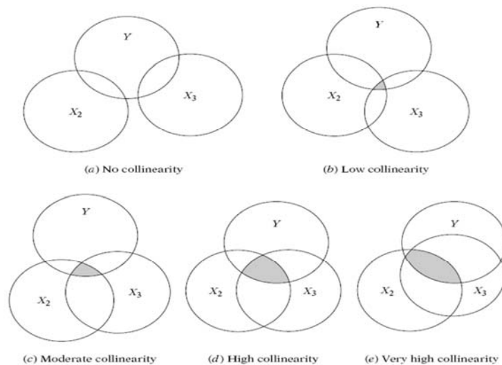
FIGURE 10.1 The Ballentine view of multicollinearity.
