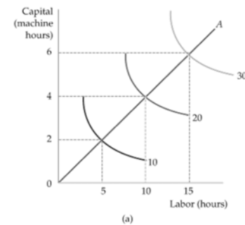
Returns to Scale
