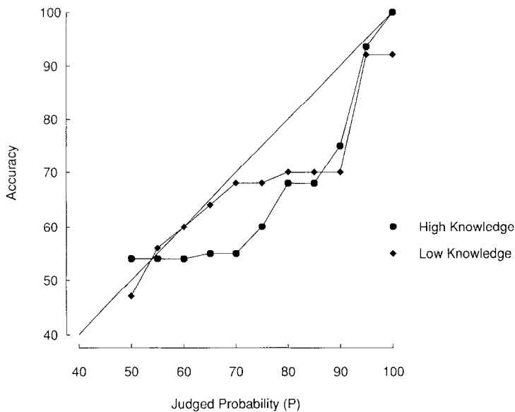
Figure 7. Calibration curves for high- and low-knowledge categories in experiment 4.
