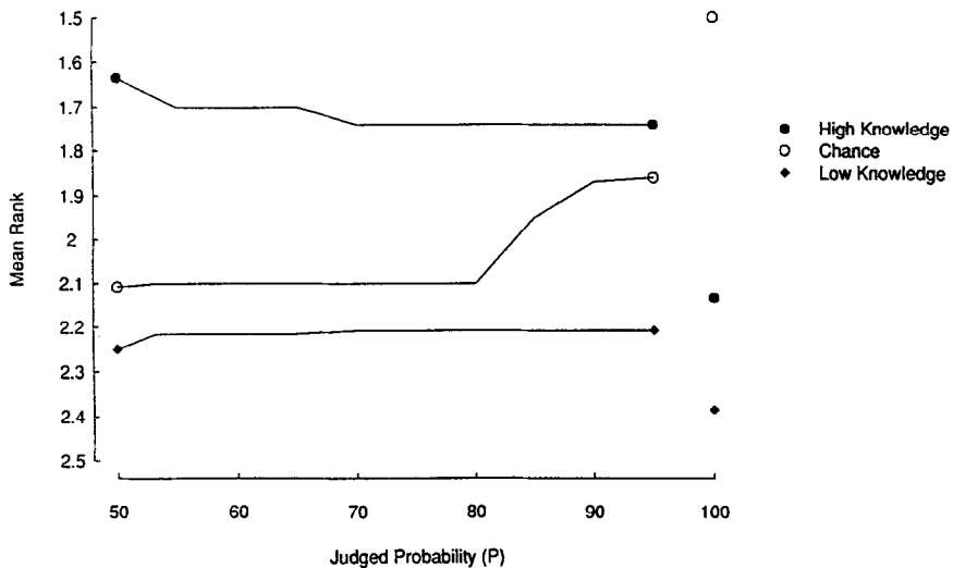
Figure 6. Ranking data for high-knowledge, low-knowledge, and chance bets as a function of P in experiment 4.
