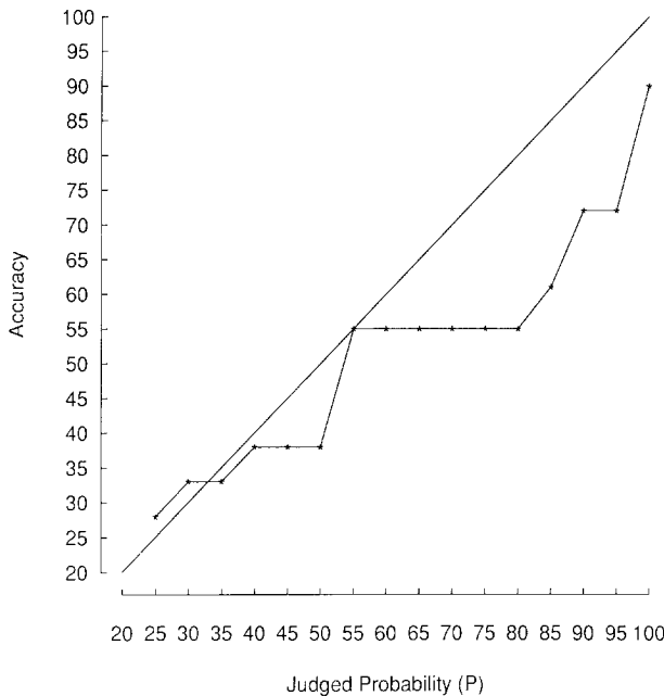
Figure 3. Calibration curve for experiment 1.
