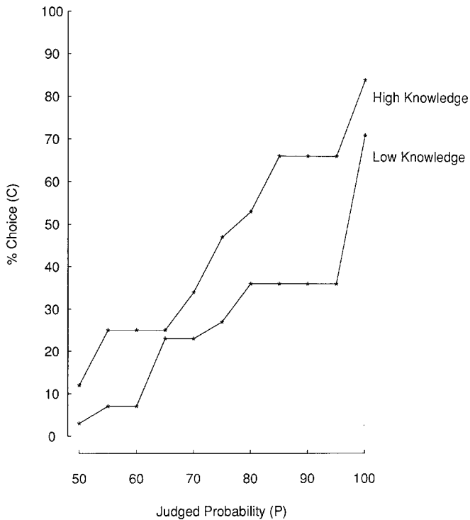
Figure 5. Percentage of choices (C) that favor a judgment bet over a matched lottery as a function of judged probability (P), for high- and low-knowledge items in experiment 2 (election data).
