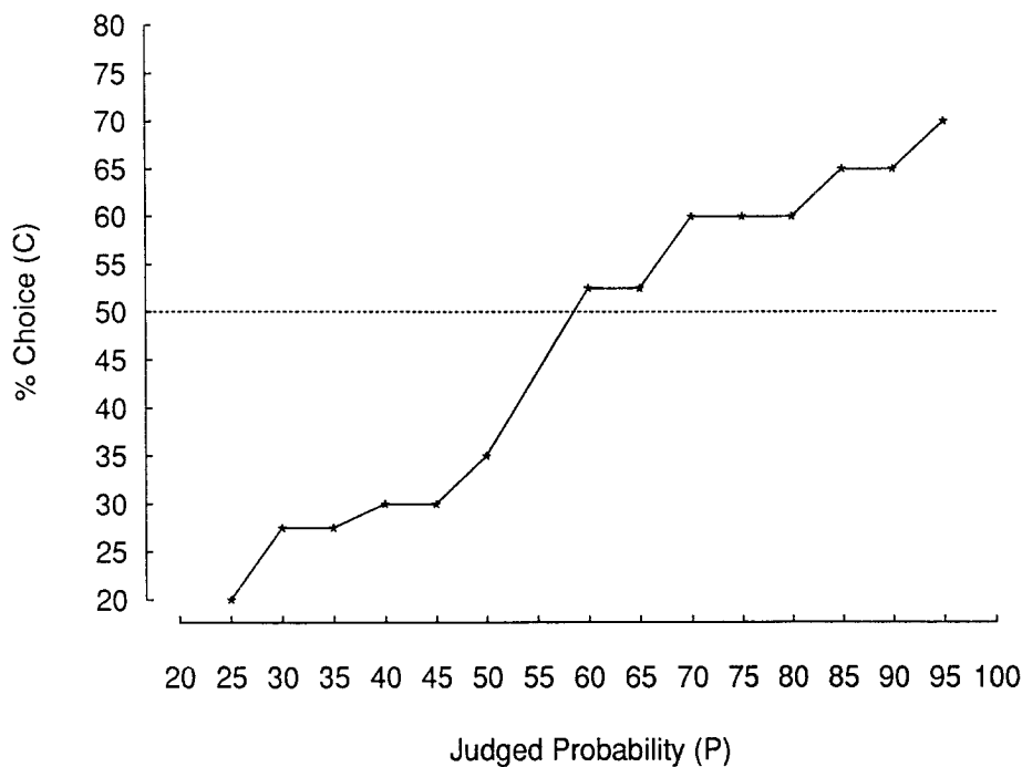
Figure 2. Percentage of choice (C) that favor a judgment bet over a matched lottery as a function of judged probability (P) in experiment 1.
