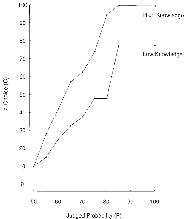
Figure 4. Percentage of choices (C) that favor a judgment bet over a matched lottery as a function of judged probability (P), for high- and low-knowledge items in the football prediction task (experiment 2).
