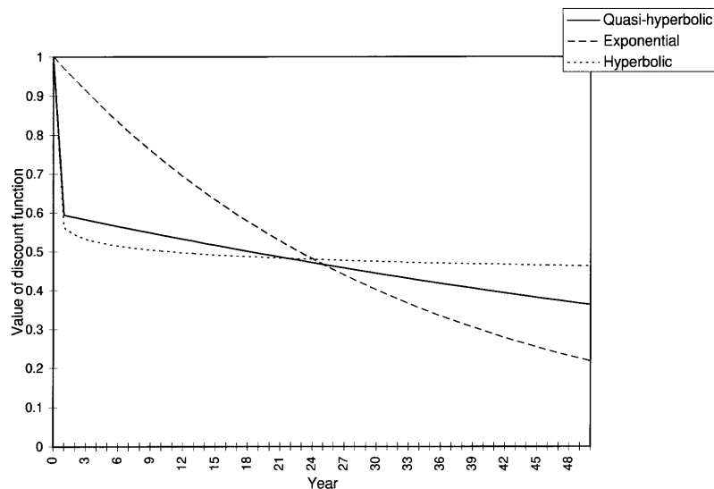
FIGURE I Discount Functions
