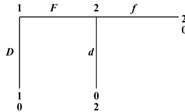
Fig. 6. Game \Gamma_6 .
