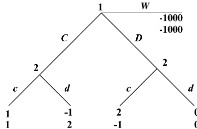
Fig. 3. Game \Gamma_3 .
