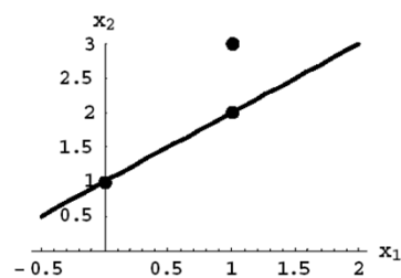
Property (b) fails
