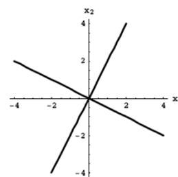
Subspaces Nul A^T and Col A
