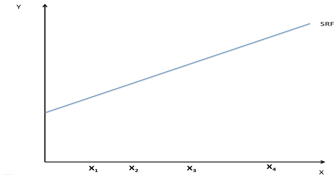
Figure 3.1: Least-Squares Criterion
