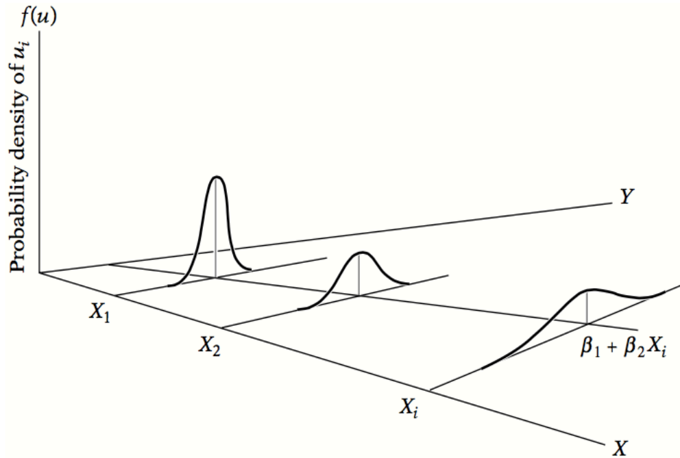
Figure 3.6: Heteroscedasticity
