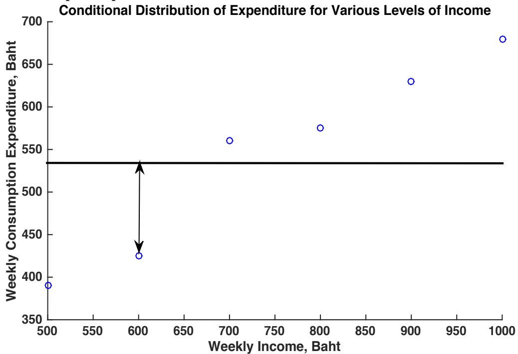
Figure 3.8: Graphic Representation
