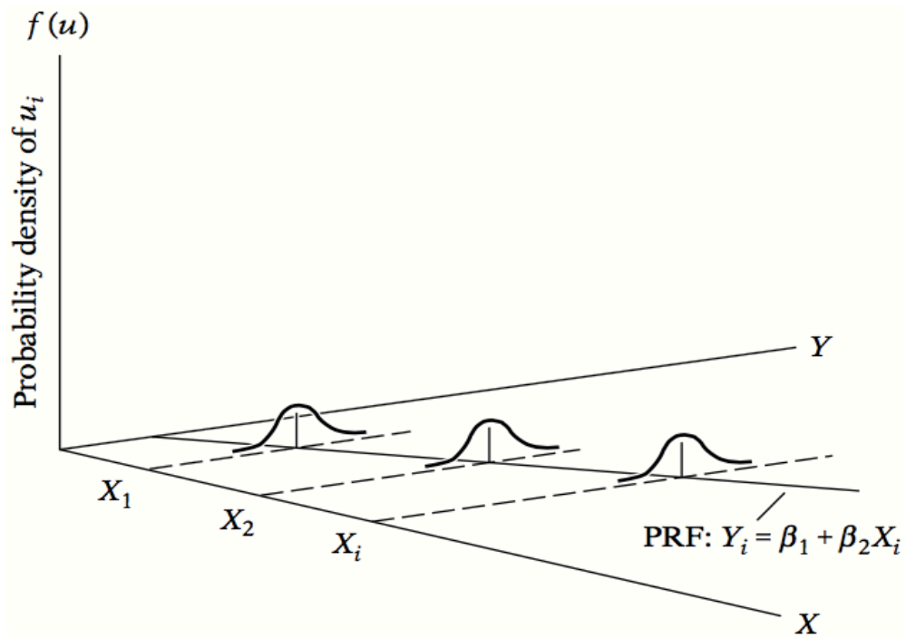
Figure 3.5: Homoscedasticity
