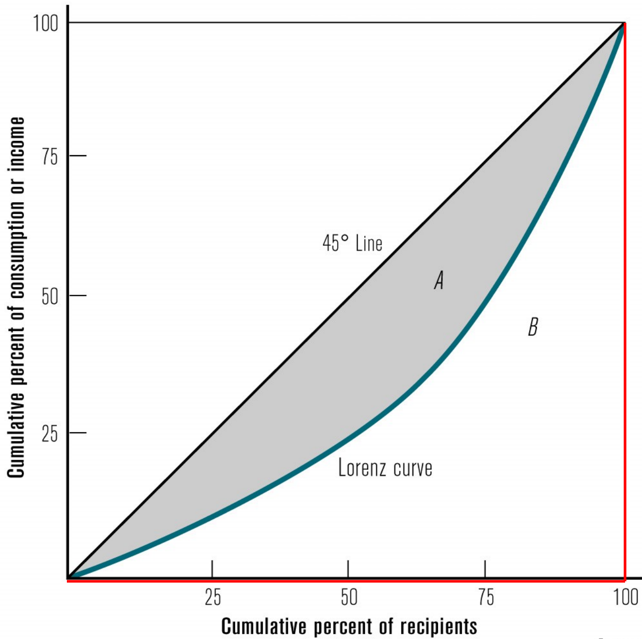
FIGURE 6.2 Lorenz Curve
