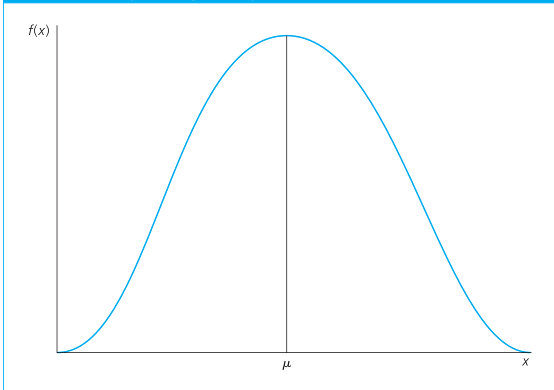
FIGURE B.3 A symmetric probability distribution.
