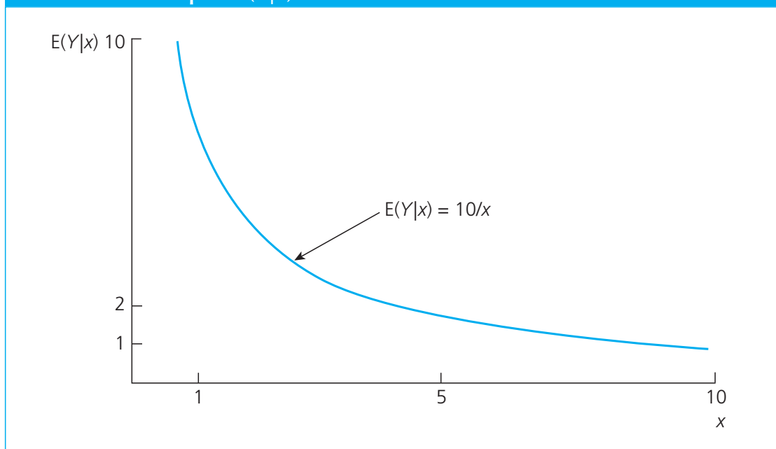
FIGURE B.6 Graph of E(Y|x) = 10/x .
