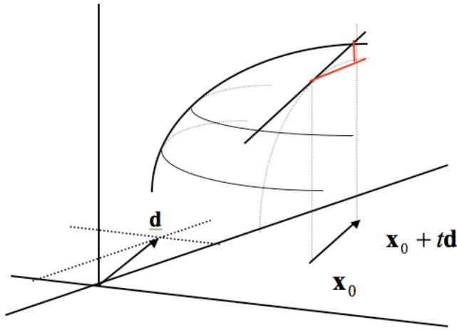
Figure 4.2 Directional derivative of f at \mathbf{x}_0 in the direction \mathbf{d} and the graph of g(t) .
