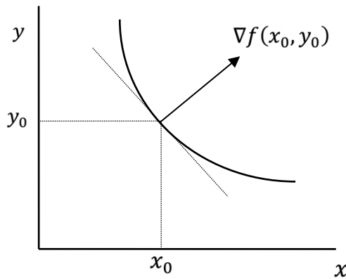
Figure 4.3 The gradient \nabla f(x_0, y_0) and the tangent line of the level set at (x_0, y_0) are orthogonal.
