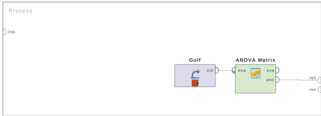
Figure 4.78: Tutorial process 'ANOVA matrix of the Golf data set'.
