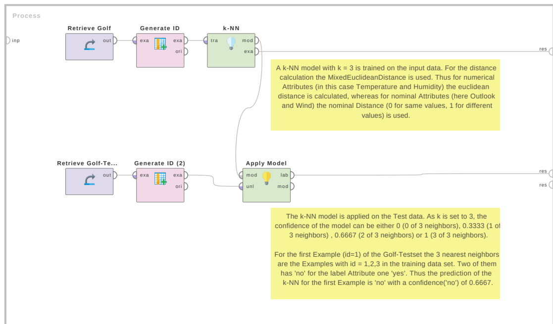
Figure 4.6: Tutorial process 'Classification of the Golf-Testset data set using the K-NN Operator'.
