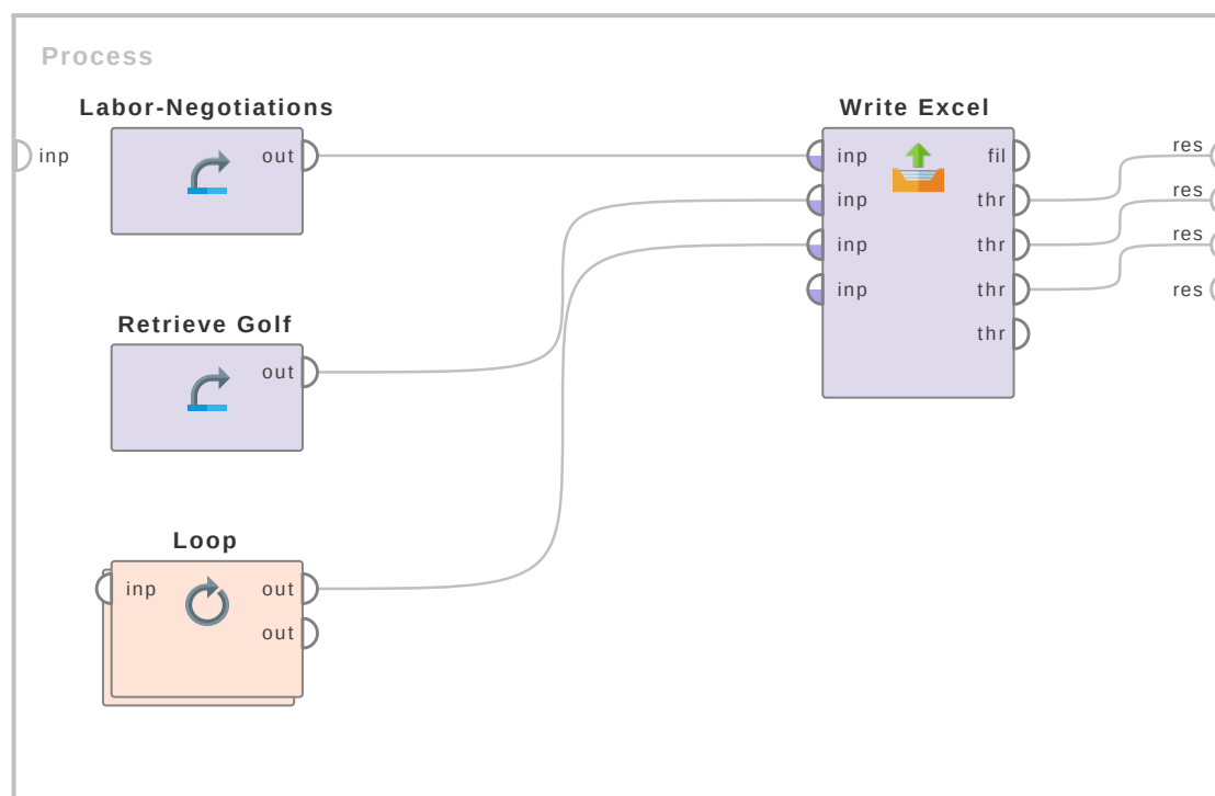
Figure 1.18: Tutorial process ‘Writing multiple data sets into one Excel file’.
