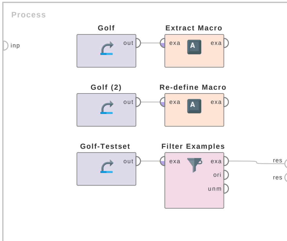
Figure 7.49: Tutorial process 'Redefining a macro using the Extract Macro operator'.
