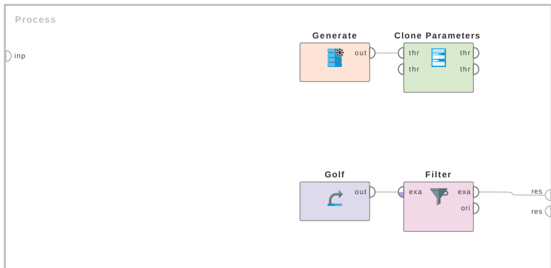
Figure 4.103: Tutorial process 'Introduction to the Clone Parameters operator'.
