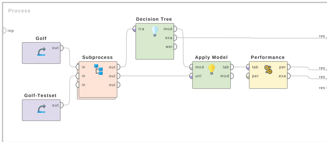
Figure 7.45: Tutorial process 'Introduction to collections'.
