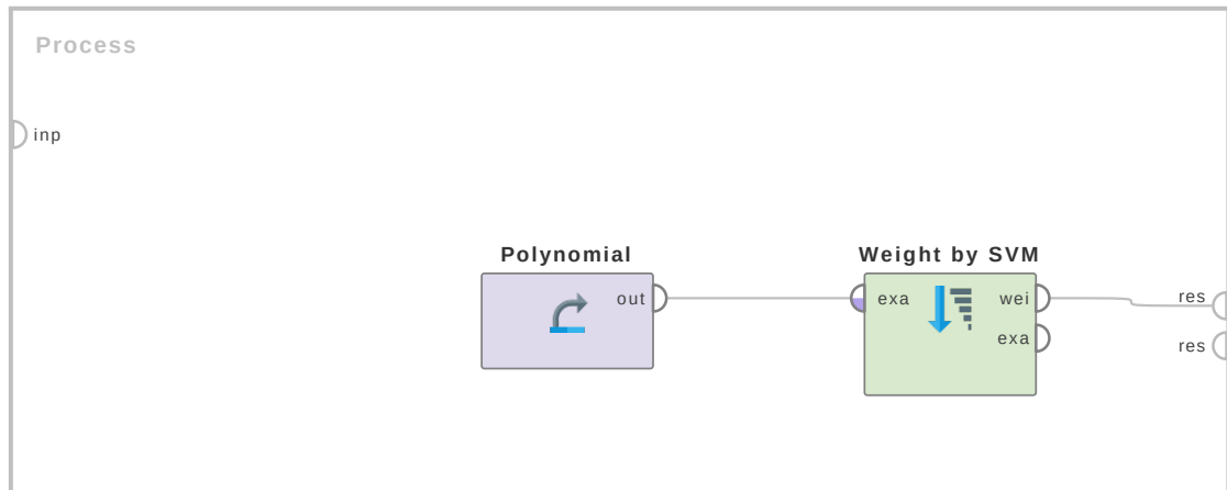
Figure 4.98: Tutorial process 'Calculating the weights of the attributes of the Polynomial data set'.
