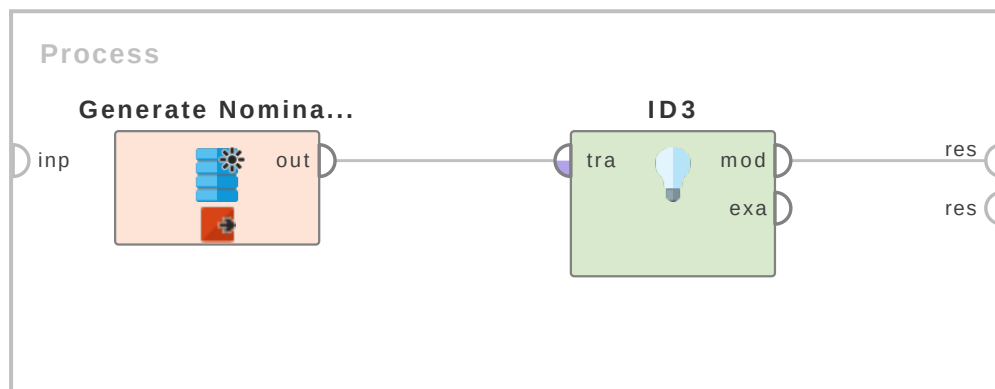
Figure 4.21: Tutorial process 'Getting started with ID3'.
