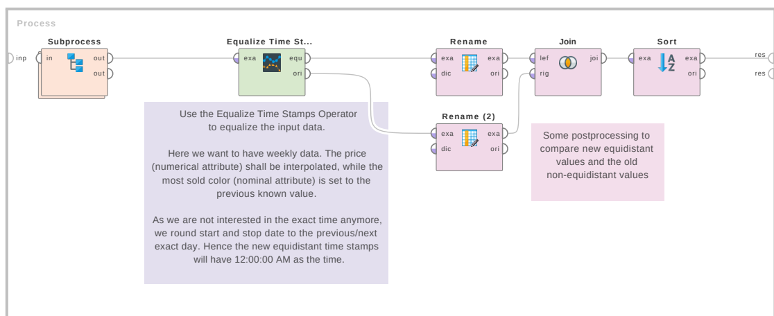
Figure 4.122: Tutorial process 'Equalize Artificial Demo Price Data'.
