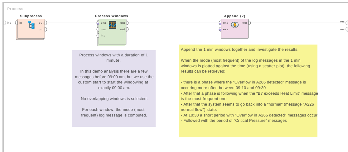
Figure 4.150: Tutorial process 'Analyzing asynchronous log data with time based windowing'.
