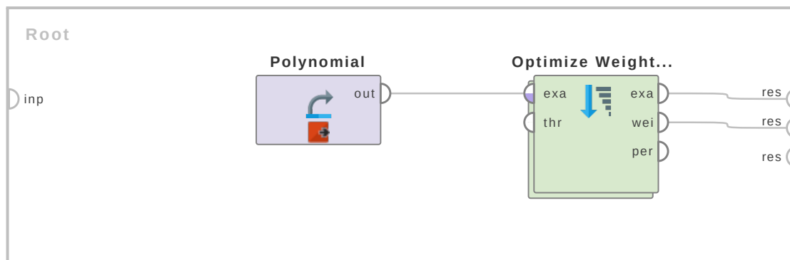
Figure 4.116: Tutorial process 'Calculating the weights of the attributes of the Polynomial data set'.
