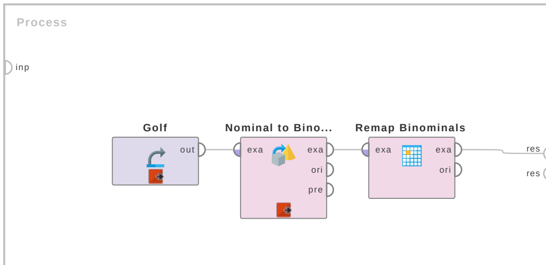
Figure 2.73: Tutorial process 'Changing mapping of the Wind attribute of the Golf data set'.
