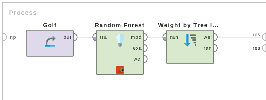
Figure 4.99: Tutorial process 'Calculating the attribute weights of the Golf data set using Random Forest model'.
