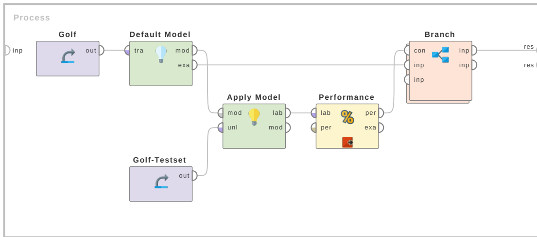
Figure 7.41: Tutorial process 'Applying different subprocesses on Golf data set depending upon the performance value'.
