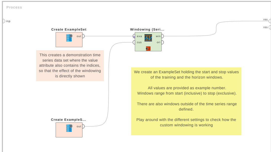
Figure 4.154: Tutorial process 'Custom Example Based Windowing of the Demo Data Set'.
