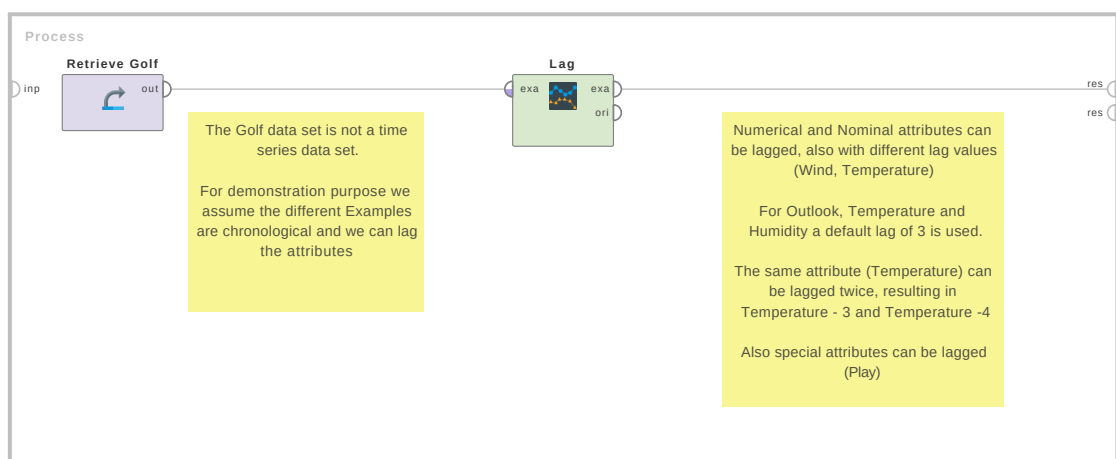
Figure 4.131: Tutorial process 'Lagging options demonstrated on the Golf data set'.
