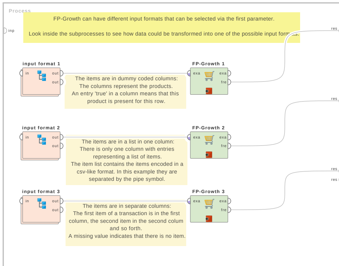
Figure 4.76: Tutorial process 'The input formats of the FP-Growth Operator'.
