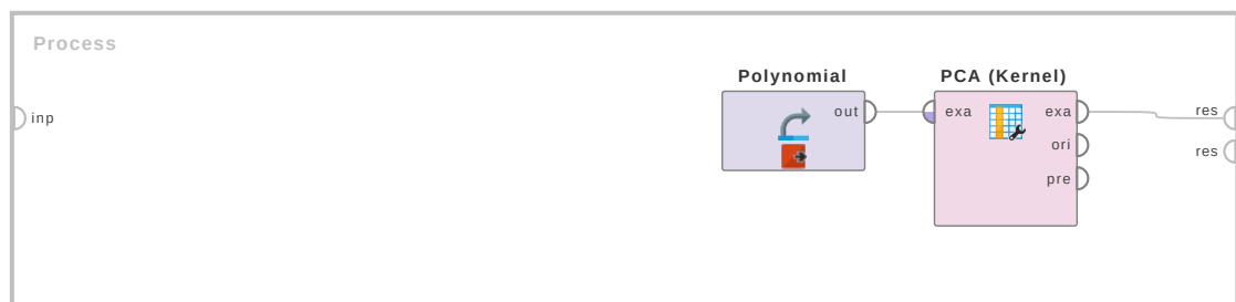
Figure 3.20: Tutorial process ‘Introduction to the Principal Component Analysis (Kernel) operator’.
