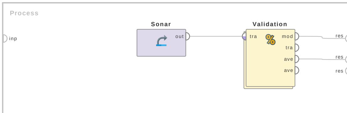
Figure 4.55: Tutorial process 'Using the Bayesian Boosting operator for generating a better Decision Tree'.
