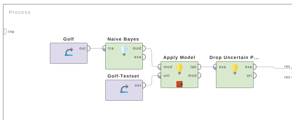
Figure 5.4: Tutorial process 'Dropping uncertain predictions of the Naive Bayes operator'.
