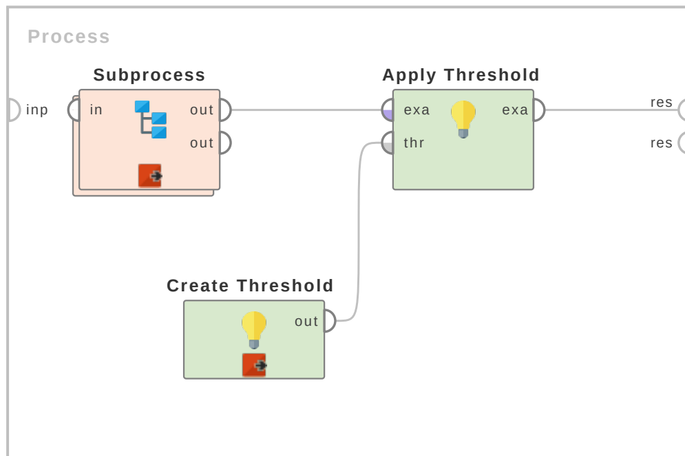
Figure 5.3: Tutorial process 'Creating and Applying thresholds'.
