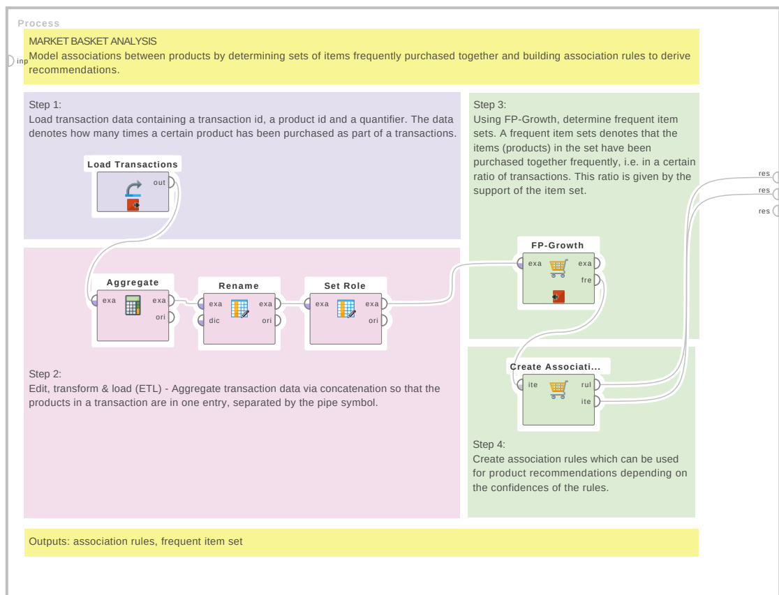
Figure 4.75: Tutorial process 'Introduction to the FP-Growth Operator'.
