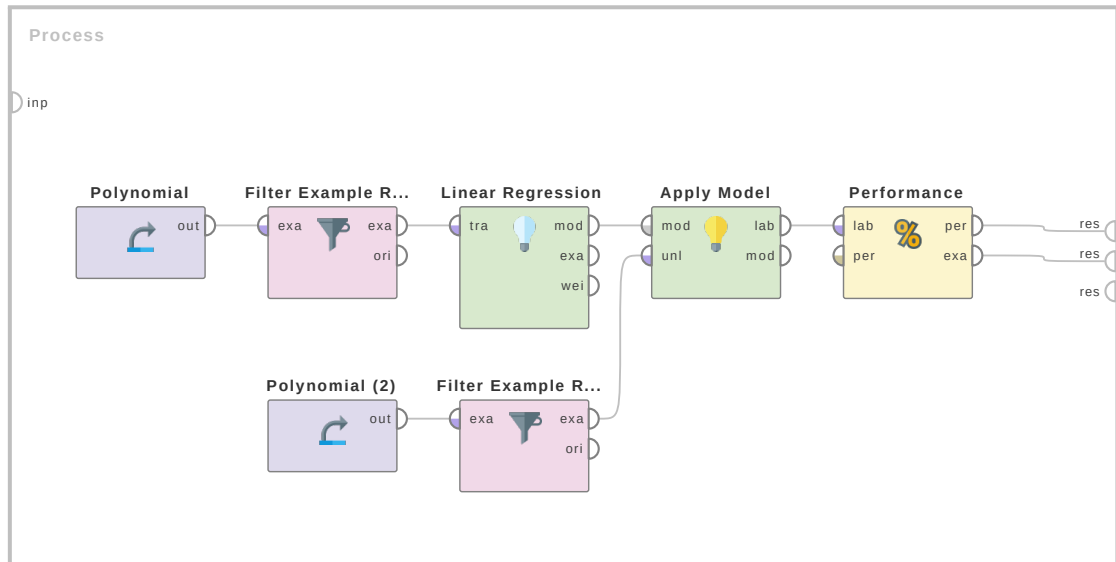
Figure 4.37: Tutorial process 'Applying the Linear Regression operator on the Polynomial data set'.
