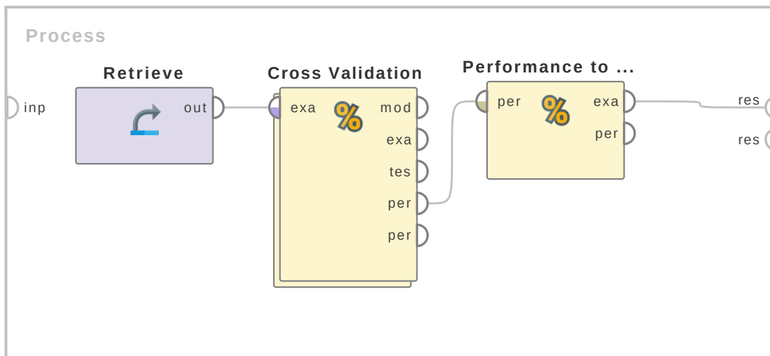
Figure 6.13: Tutorial process 'Assessing the performance of a prediction'.
