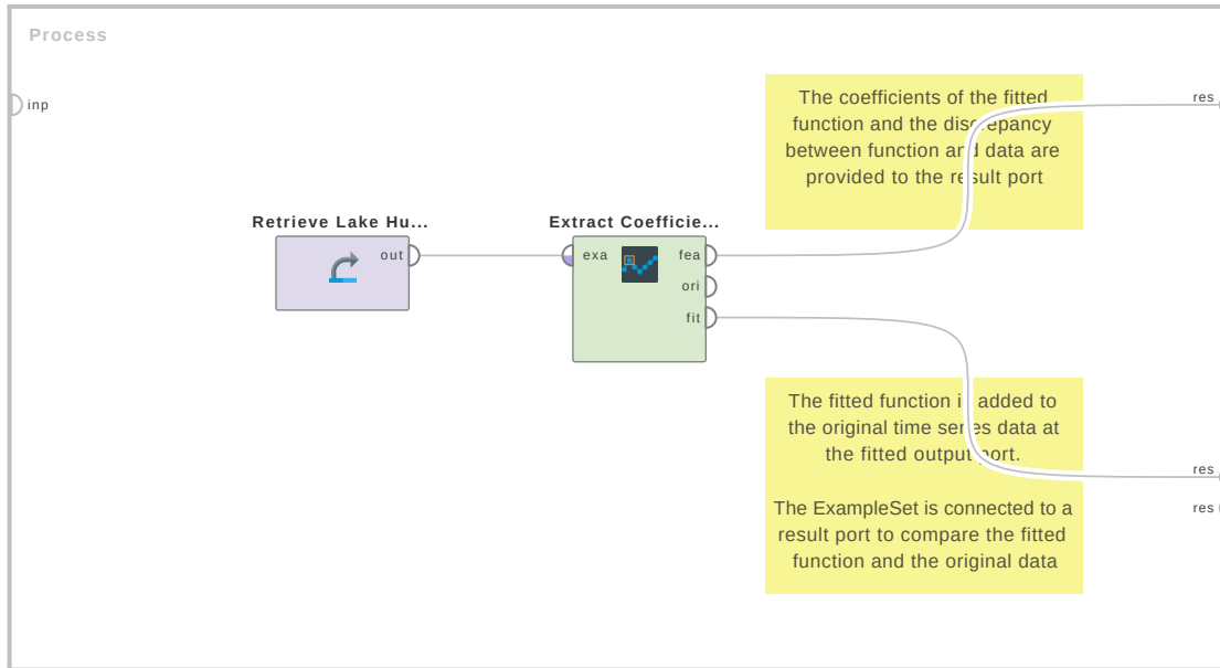
Figure 4.144: Tutorial process 'Fitting a parabola to Lake Huron time series'.
