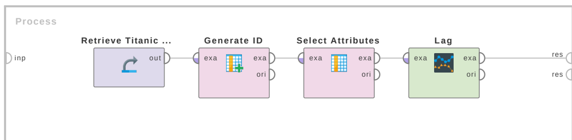
Figure 4.132: Tutorial process 'Positive and Negative lags demonstrated on the Titanic data set'.
