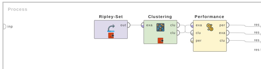
Figure 6.23: Tutorial process ‘Evaluating the performance of the K-Medoids clustering model’.
