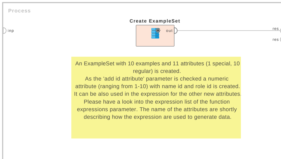
Figure 7.74: Tutorial process 'Usage of the attribute functions generator'.
