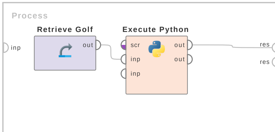
Figure 7.12: Tutorial process 'Meta data handling'.
