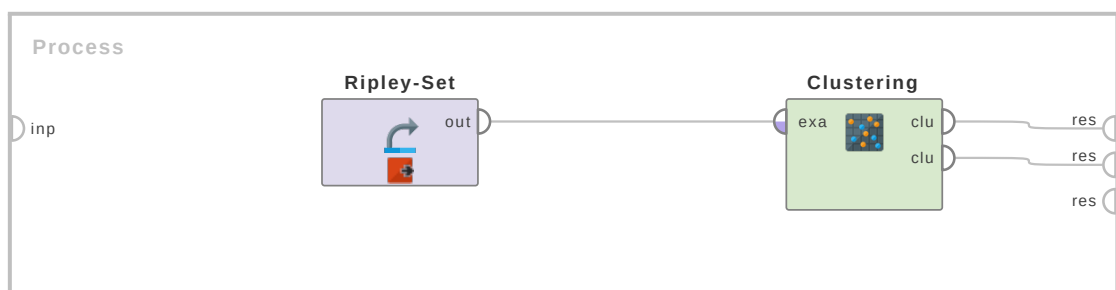
Figure 4.67: Tutorial process 'Random clustering of the Ripley-Set data set'.
