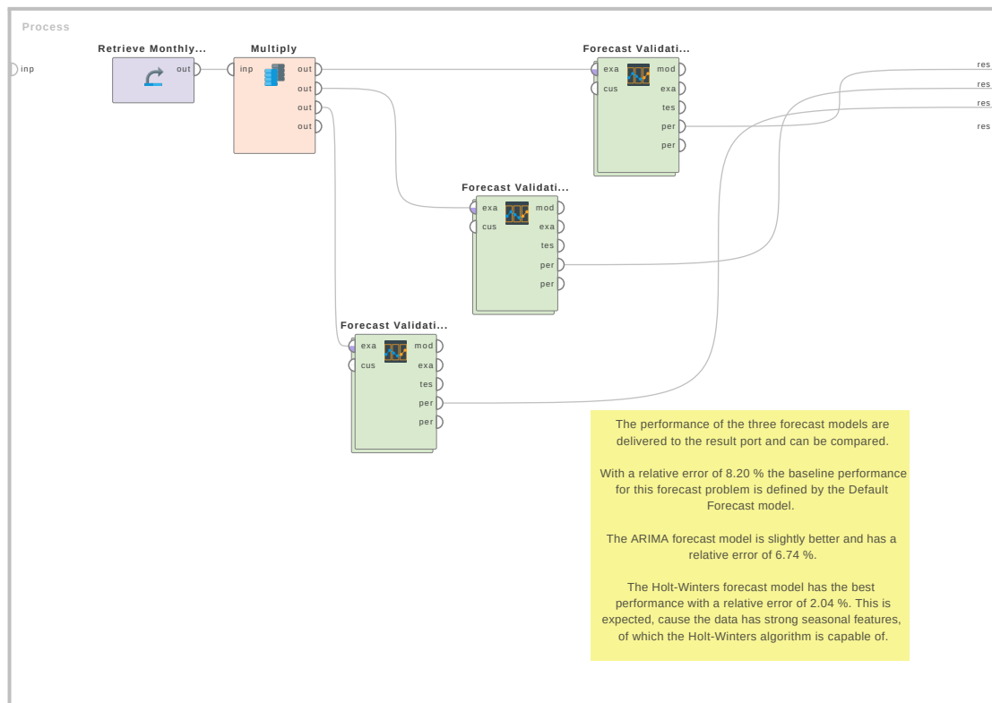
Figure 4.161: Tutorial process 'Compare Performance of Forecast Models on Milk Production Data'.
