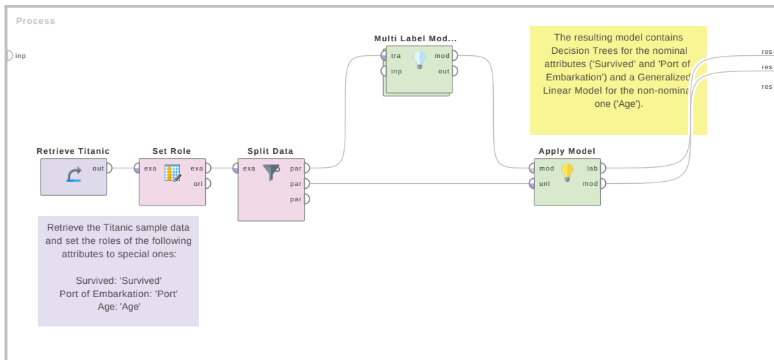
Figure 4.59: Tutorial process 'Training different models for different types of label attributes'.
