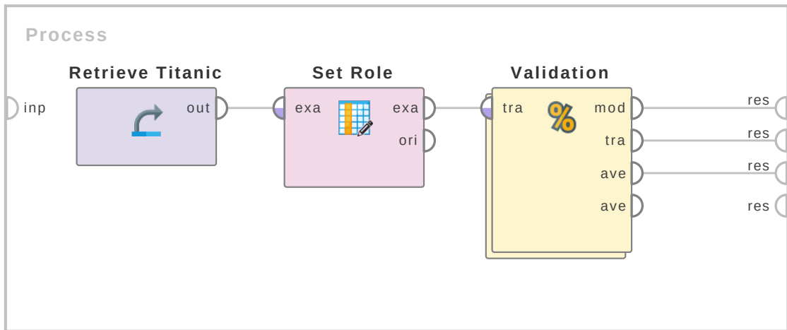
Figure 4.29: Tutorial process 'Classification with Split Validation using Deep Learning'.
