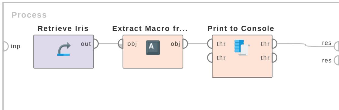
Figure 7.67: Tutorial process 'Extracting the Source annotation from an example set'.
