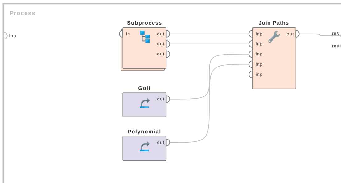
Figure 7.85: Tutorial process 'Returning the first non-null object'.
