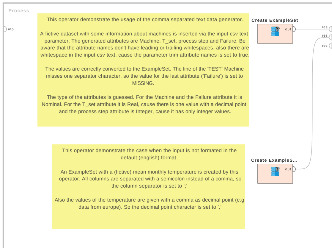
Figure 7.77: Tutorial process 'Usage of the comma separated text generator'.
