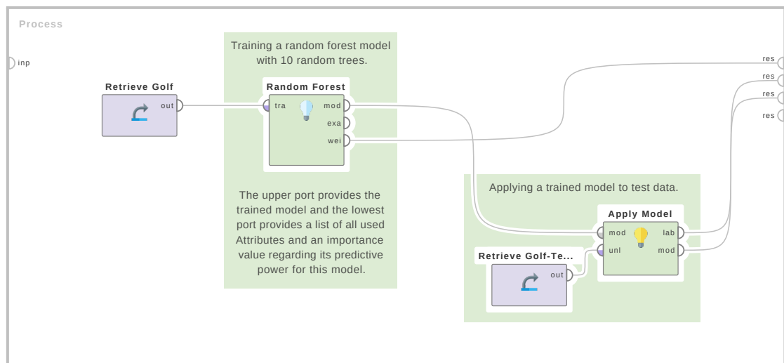
Figure 4.22: Tutorial process 'Generating a set of random trees using the random forest Operator'.
