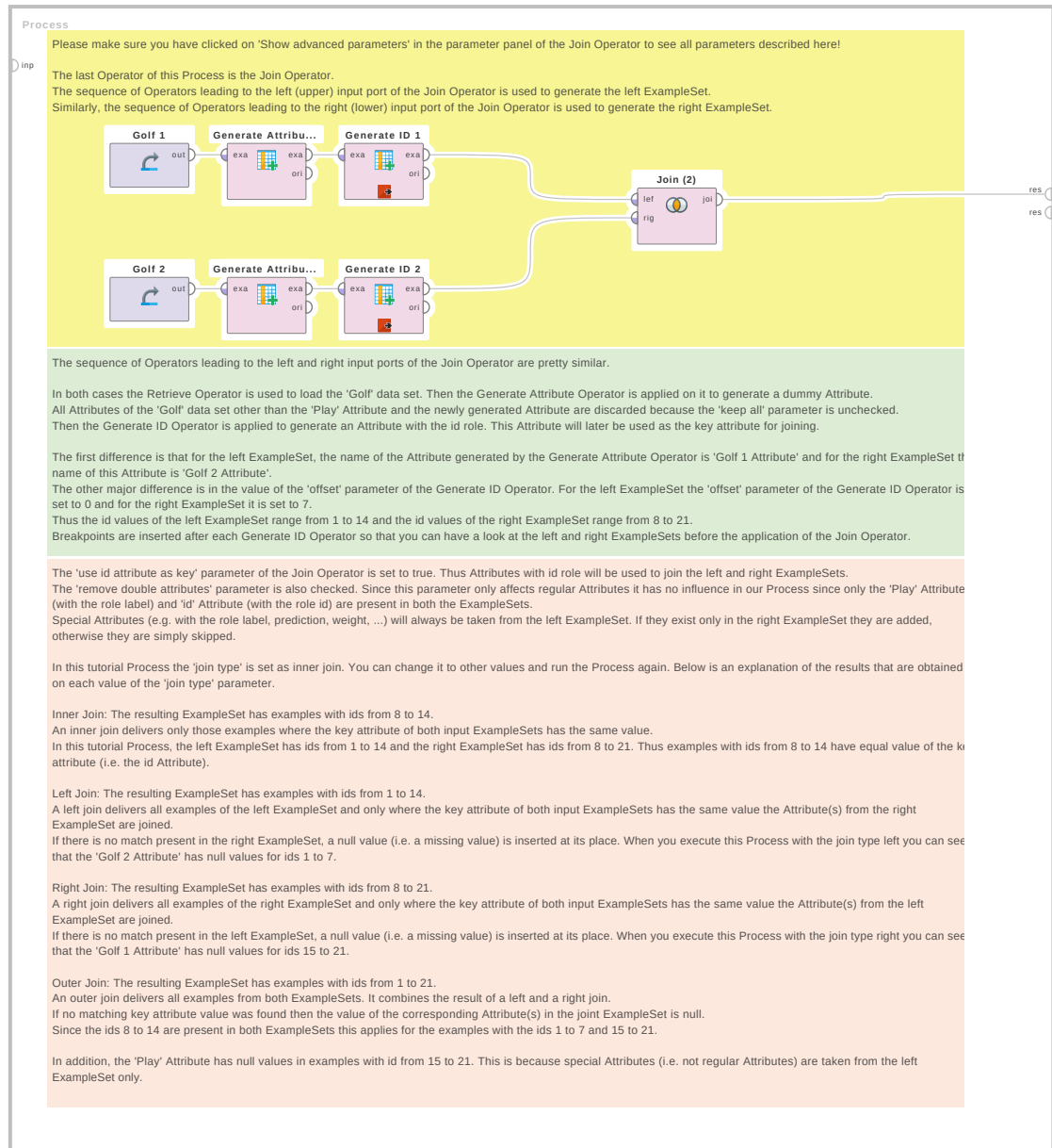
Figure 2.63: Tutorial process 'Explore the different join types'.
