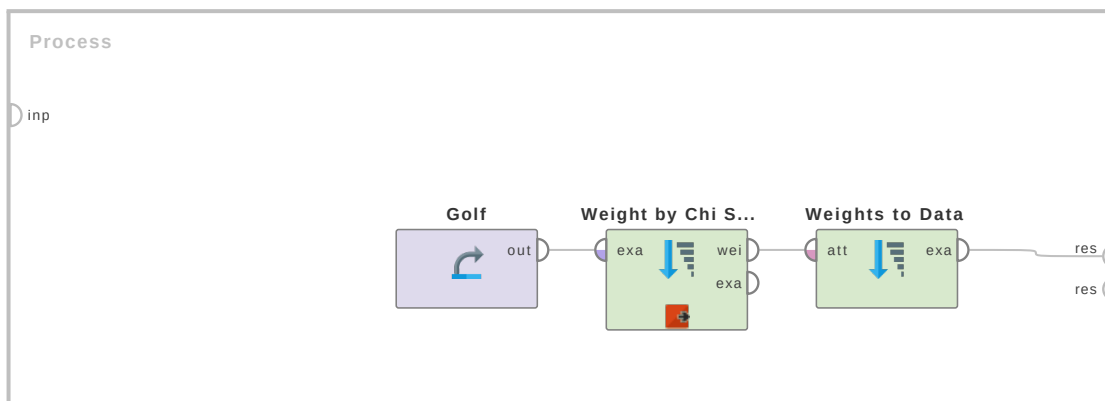
Figure 4.101: Tutorial process 'Manually setting the attribute weights of the Golf data set'.
