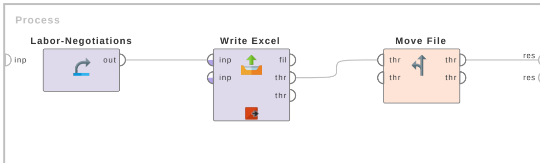
Figure 7.60: Tutorial process 'Writing the Labor-Negotiations data set into an Excel file and moving it'.
