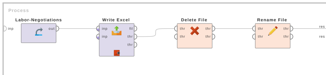
Figure 7.61: Tutorial process 'Writing the Labor-Negotiations data set into an Excel file and re-naming it'.
