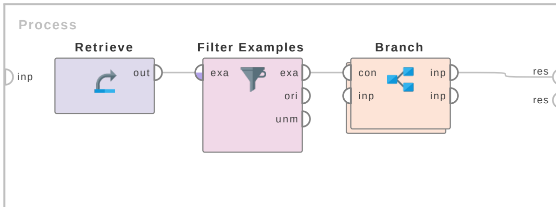
Figure 7.47: Tutorial process ‘Throw exeption if no examples passed’.
