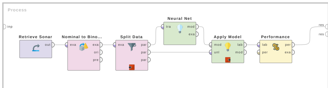
Figure 6.15: Tutorial process ‘Separate mines from rocks’.
