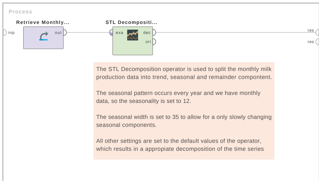
Figure 4.141: Tutorial process 'STL Decomposition of the monthly milk production data set'.
