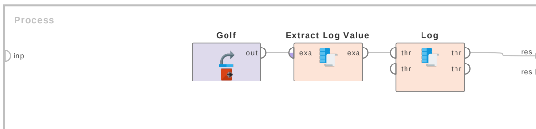
Figure 7.68: Tutorial process 'Logging the value of an attribute by Extract Log Value operator'.
