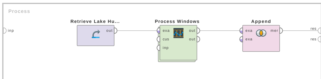
Figure 4.142: Tutorial process 'Extract Aggregates of the Lake Huron data set'.
