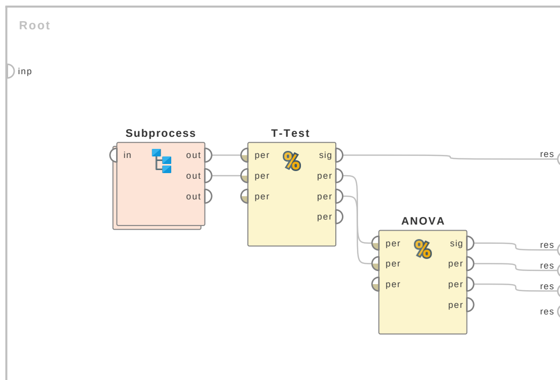
Figure 6.27: Tutorial process ‘Comparison of performance vectors using statistical significance tests’.
