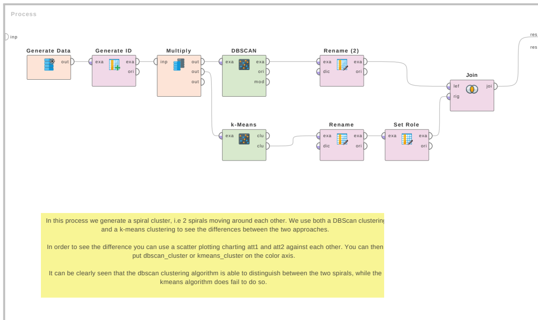
Figure 4.64: Tutorial process 'Clustering Spiral Clusters'.
