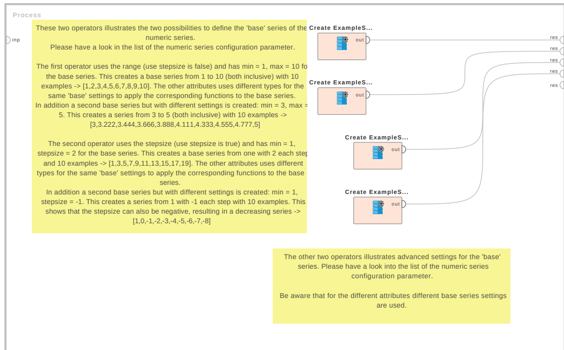
Figure 7.75: Tutorial process 'Usage of the numeric series generator'.
