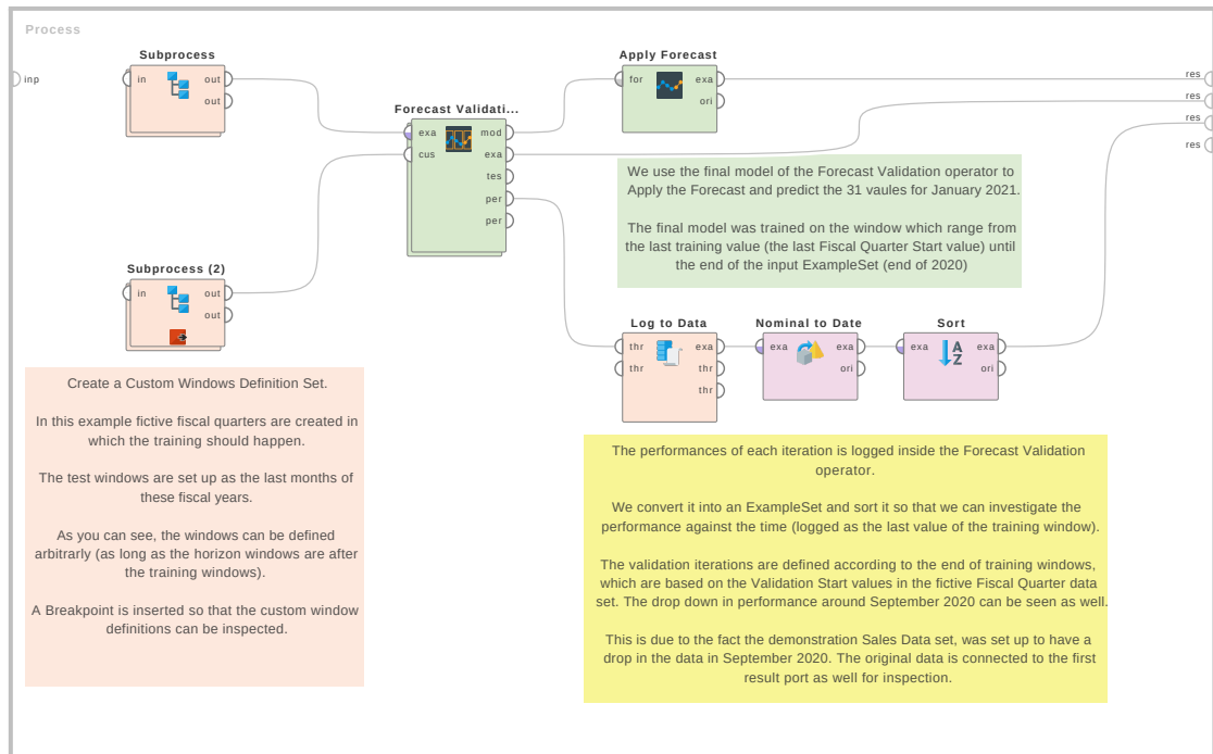
Figure 4.167: Tutorial process 'Use custom windowing to define your own training and test windows'.
