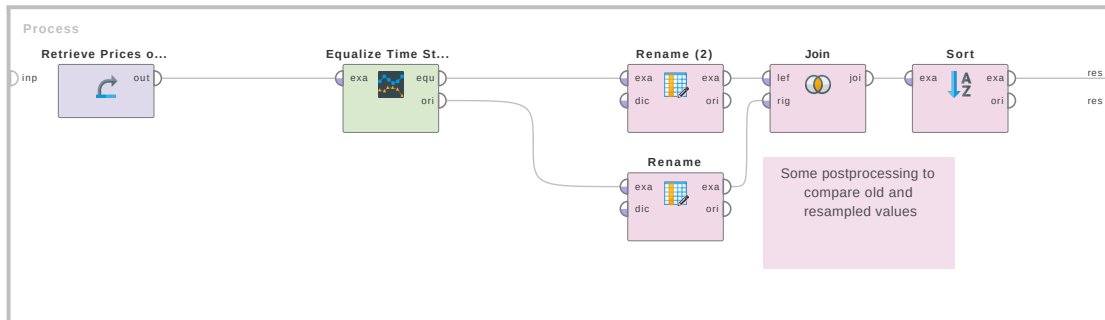
Figure 4.123: Tutorial process 'Resample Gas Station Data Set to 90 minutes steps'.
