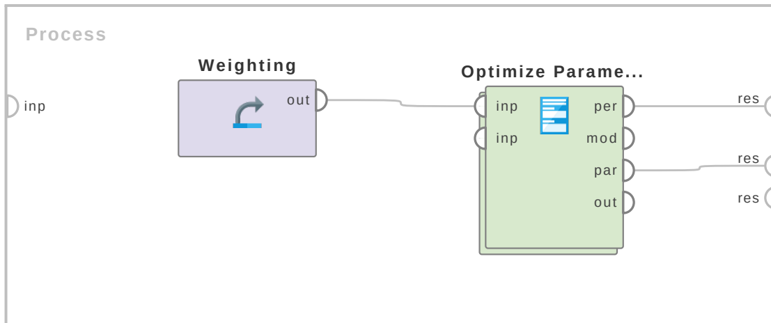
Figure 4.105: Tutorial process 'Finding optimal values of parameters of the SVM Operator'.
