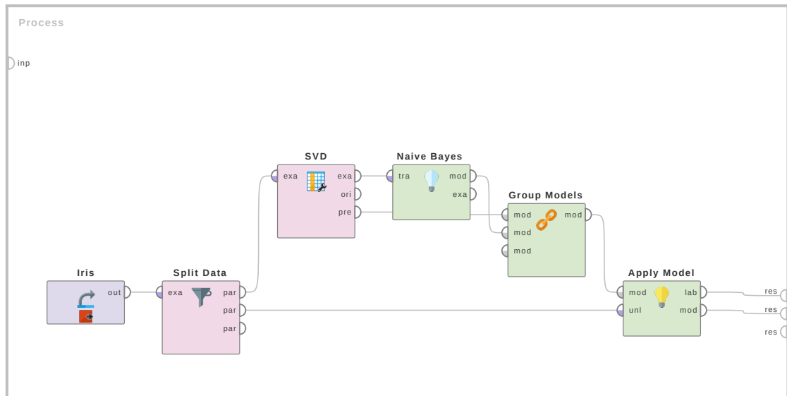
Figure 4.4: Tutorial process ‘Grouping models and applying the resultant grouped model’.
