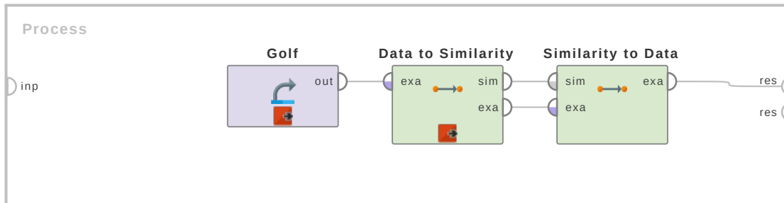
Figure 4.86: Tutorial process 'Introduction to the Similarity to Data operator'.
