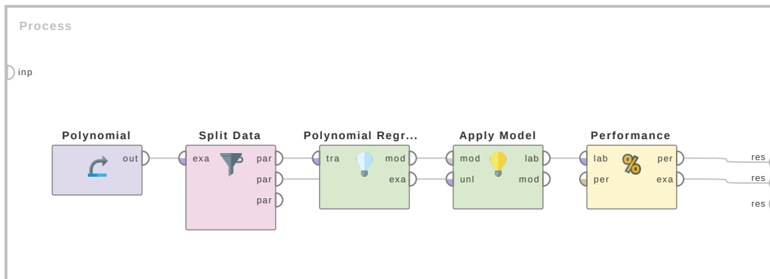
Figure 4.39: Tutorial process 'Applying the Polynomial Regression operator on the Polynomial data set'.
