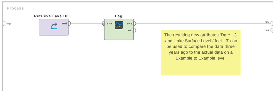
Figure 4.130: Tutorial process 'Lagging Lake Huron Data Set'.
