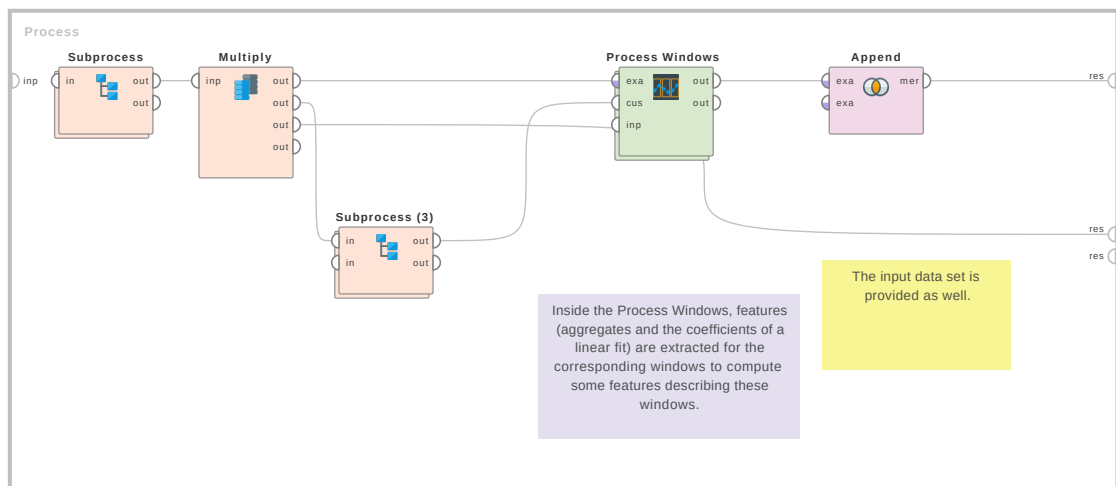
Figure 4.151: Tutorial process 'Use Extract Peaks and Custom Windowing to analysis industrial sensor data'.
