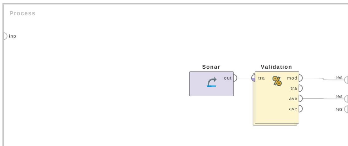
Figure 4.43: Tutorial process 'Introduction to the Logistic Regression (Evolutionary) operator'.
