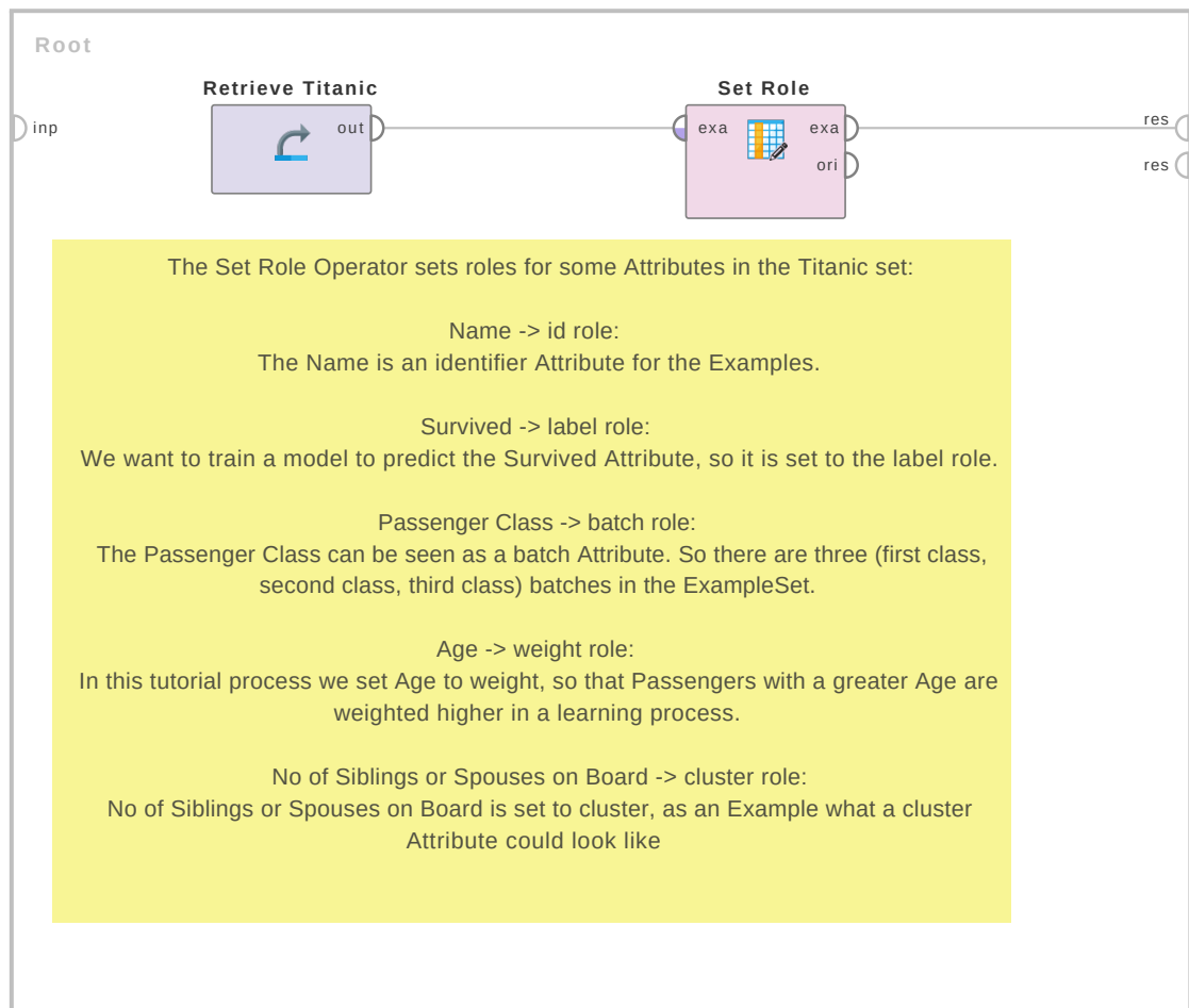
Figure 2.7: Tutorial process 'Set Role on Titanic Data Set'.
