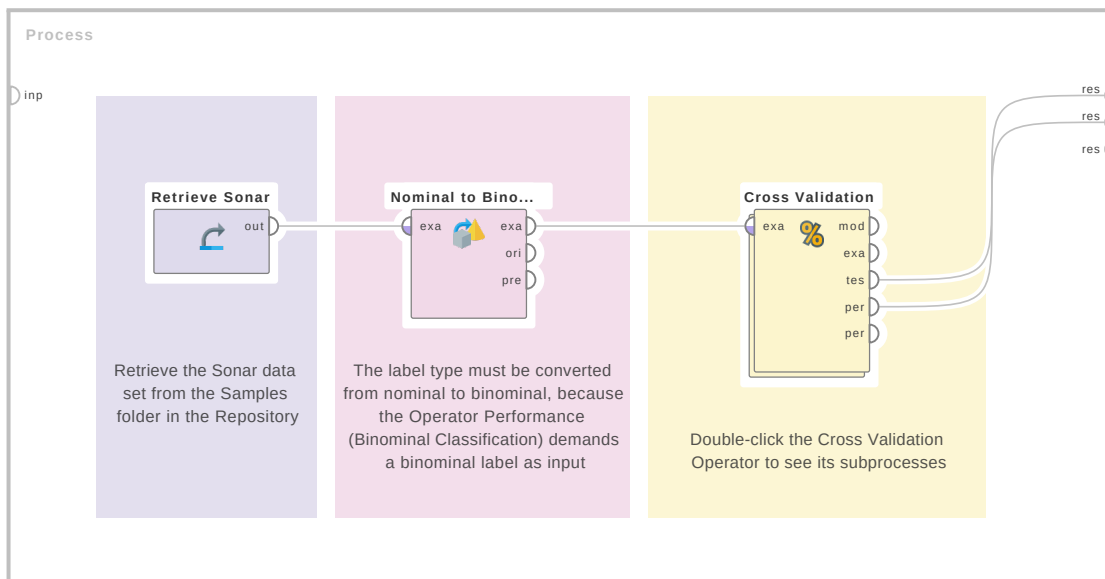
Figure 6.16: Tutorial process 'Separate mines from rocks, with Cross Validation'.
