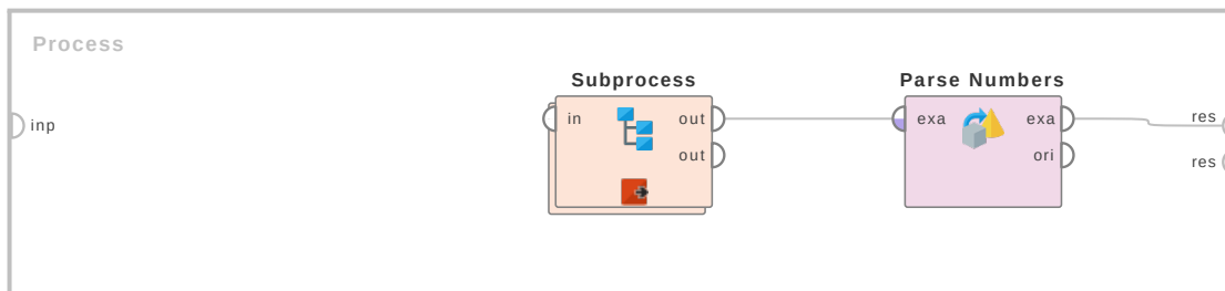
Figure 2.19: Tutorial process ‘Nominal to Numeric conversion by the Parse Numbers operator’.
