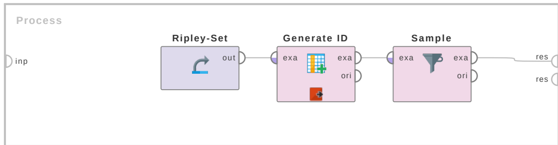
Figure 2.48: Tutorial process 'Sampling the Ripley-Set data set'.
