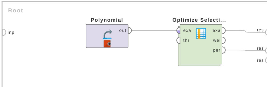
Figure 4.110: Tutorial process 'Feature reduction of the Polynomial data set'.
