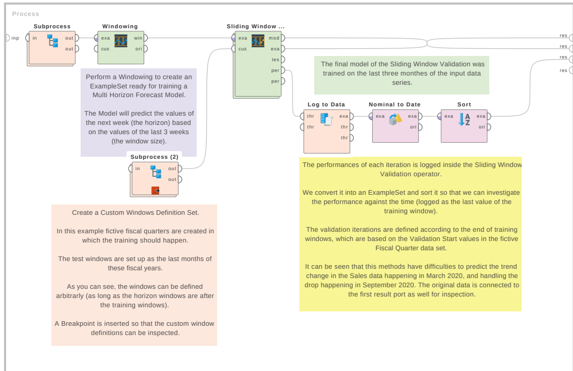
Figure 4.171: Tutorial process 'Use custom windowing to define your own training and test windows'.
