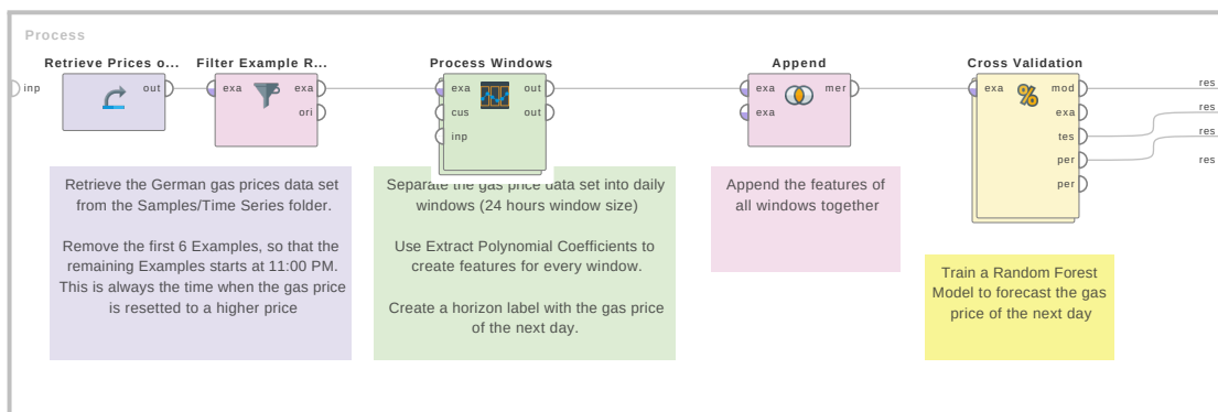
Figure 4.145: Tutorial process 'Using fit coefficients of linear fit as features'.
