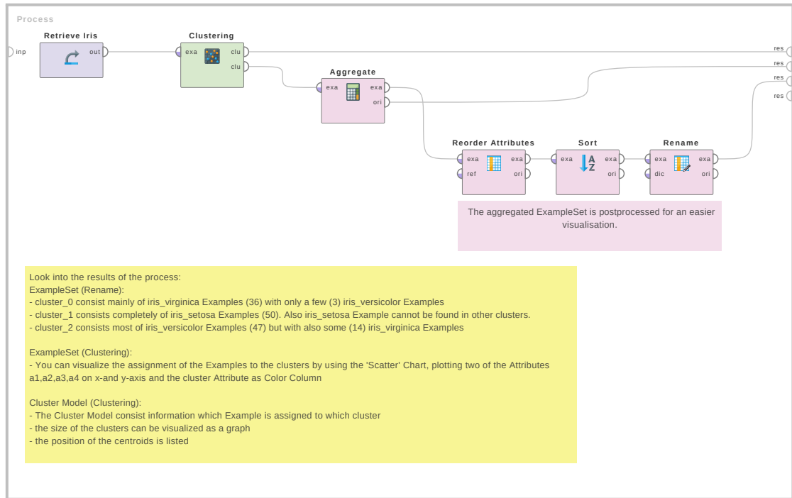
Figure 4.70: Tutorial process 'Clustering of the Iris Data Set'.
