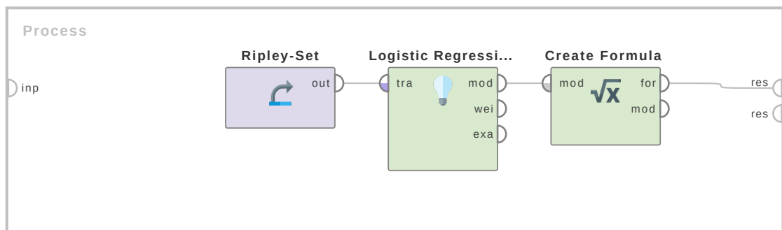
Figure 4.3: Tutorial process 'Formula of the Logistic Regression model'.
