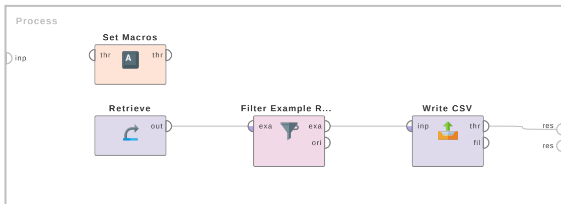
Figure 7.53: Tutorial process 'Introduction to the Set Macros operator'.
