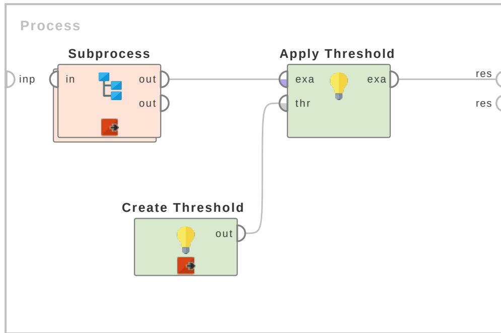
Figure 5.2: Tutorial process 'Creating and Applying thresholds'.
