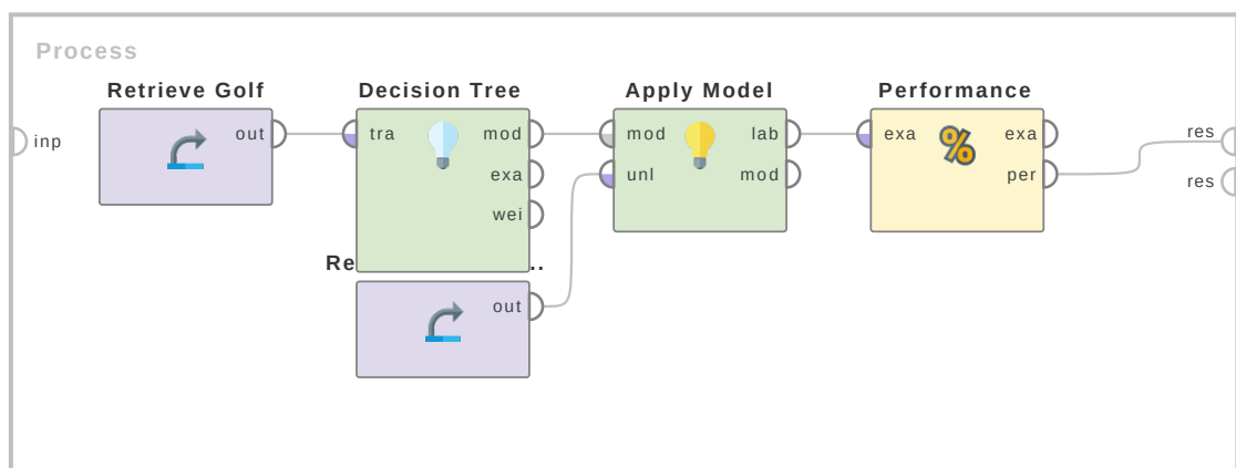
Figure 6.19: Tutorial process 'Applying the Performance (Ranking) operator on the Golf data set'.
