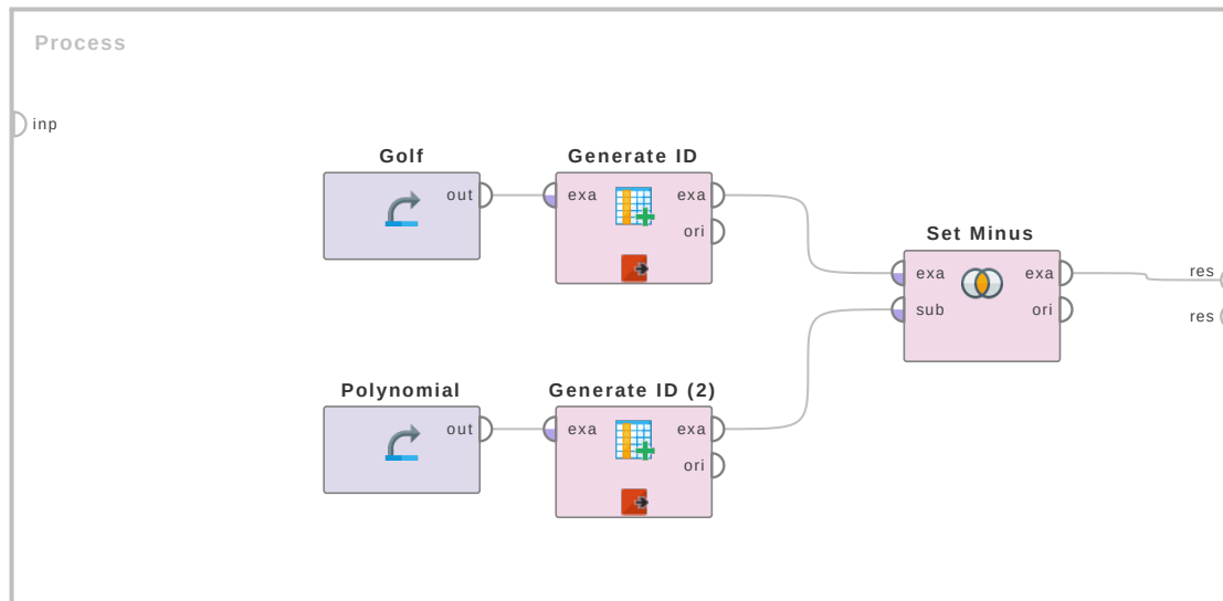
Figure 2.64: Tutorial process 'Introduction to the Set Minus operator'.
