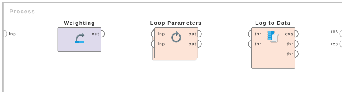
Figure 7.71: Tutorial process 'Accessing Training vs Testing error using the Log and Log to Data operators'.
