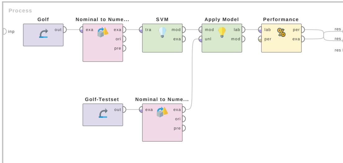
Figure 4.48: Tutorial process 'SVM with rbf kernel'.
