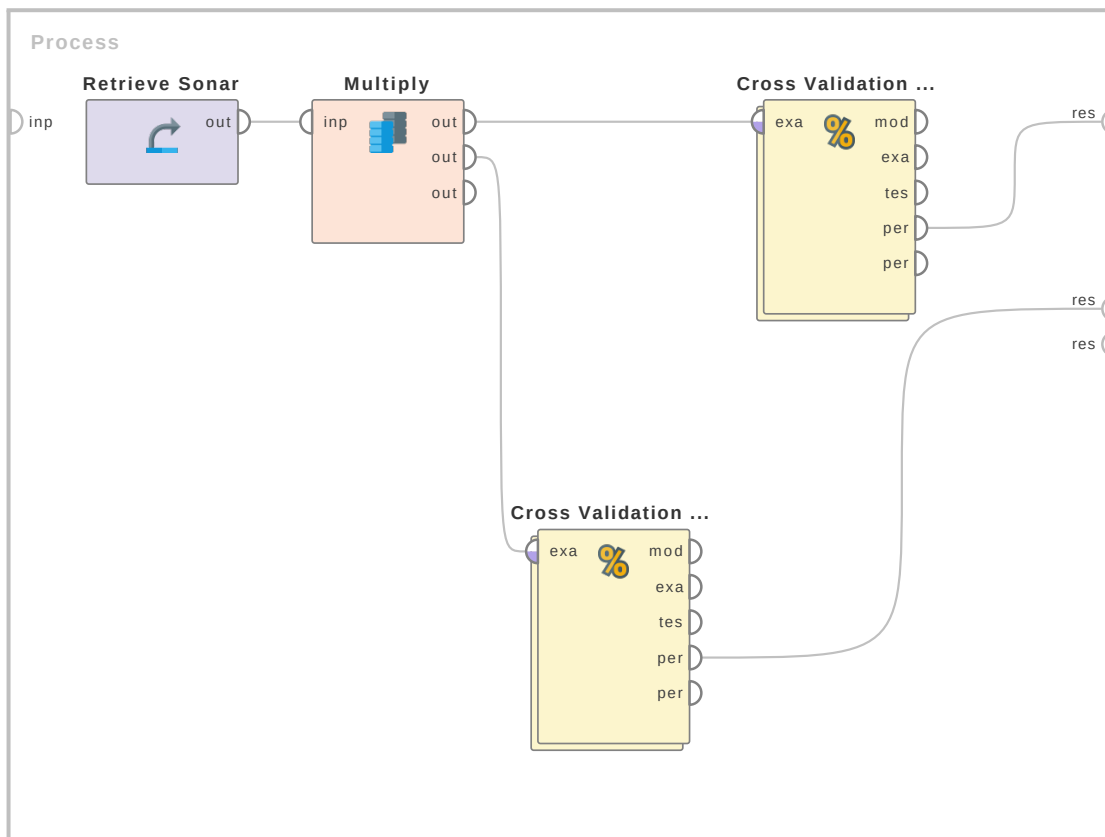
Figure 4.7: Tutorial process 'Performance difference between normalized and not normalized data'.
