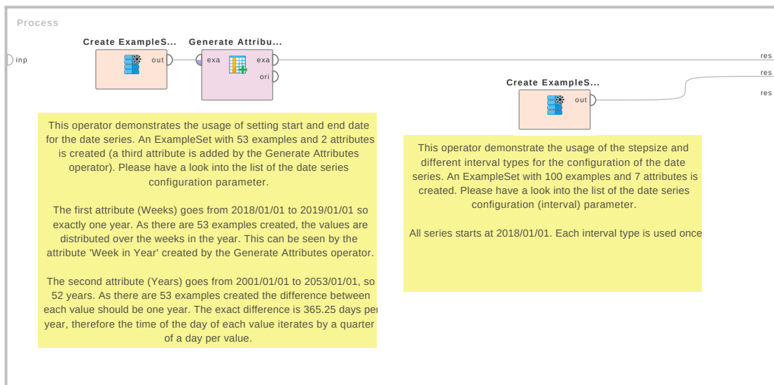
Figure 7.76: Tutorial process 'Usage of the date series generator'.
