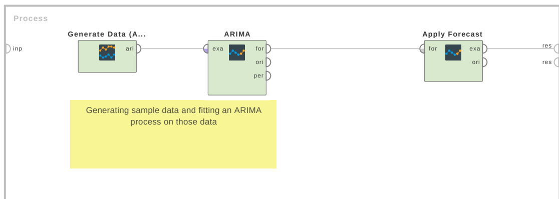
Figure 4.159: Tutorial process 'Forecasting an ARIMA process'.
