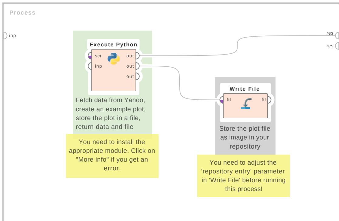
Figure 7.10: Tutorial process 'Creating a plot using Python and storing it in your repository'.
