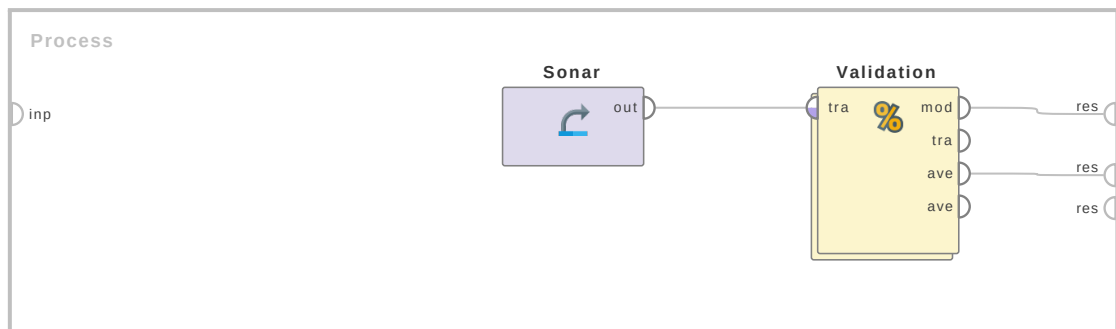
Figure 4.57: Tutorial process 'Using the MetaCost operator for generating a better Decision Tree'.
