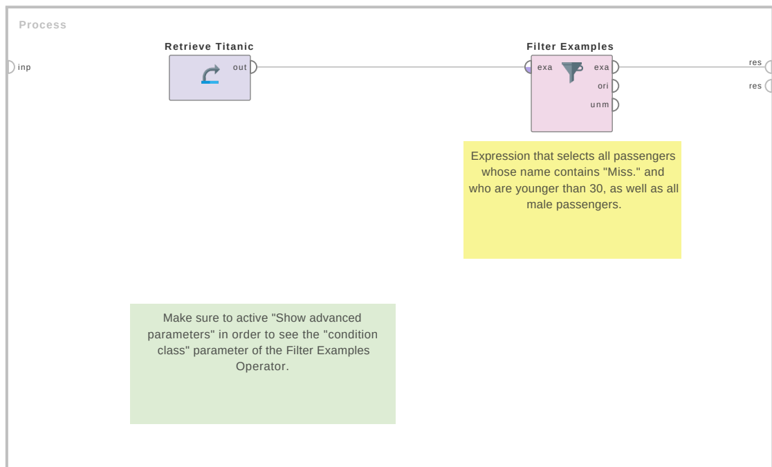
Figure 2.47: Tutorial process 'Filter Examples using expression'.
