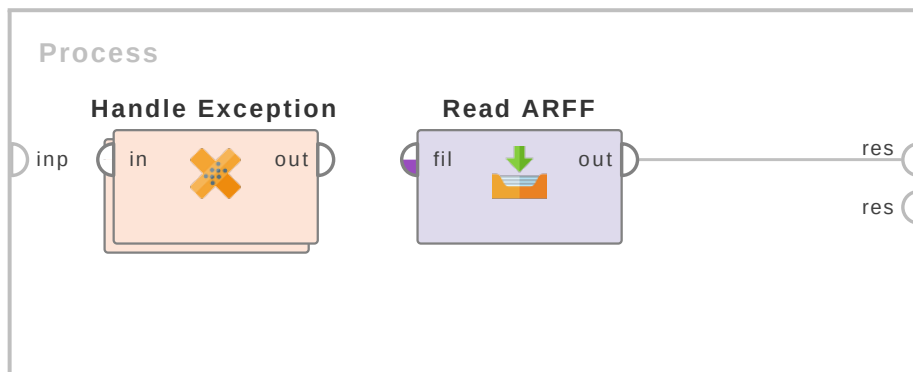
Figure 1.15: Tutorial process 'Reading an ARFF file using the Read ARFF operator'.
