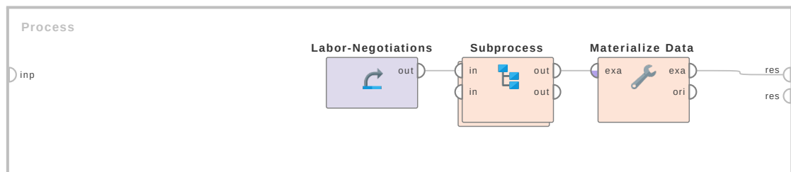
Figure 7.86: Tutorial process 'Creating fresh copy of an ExampleSet'.
