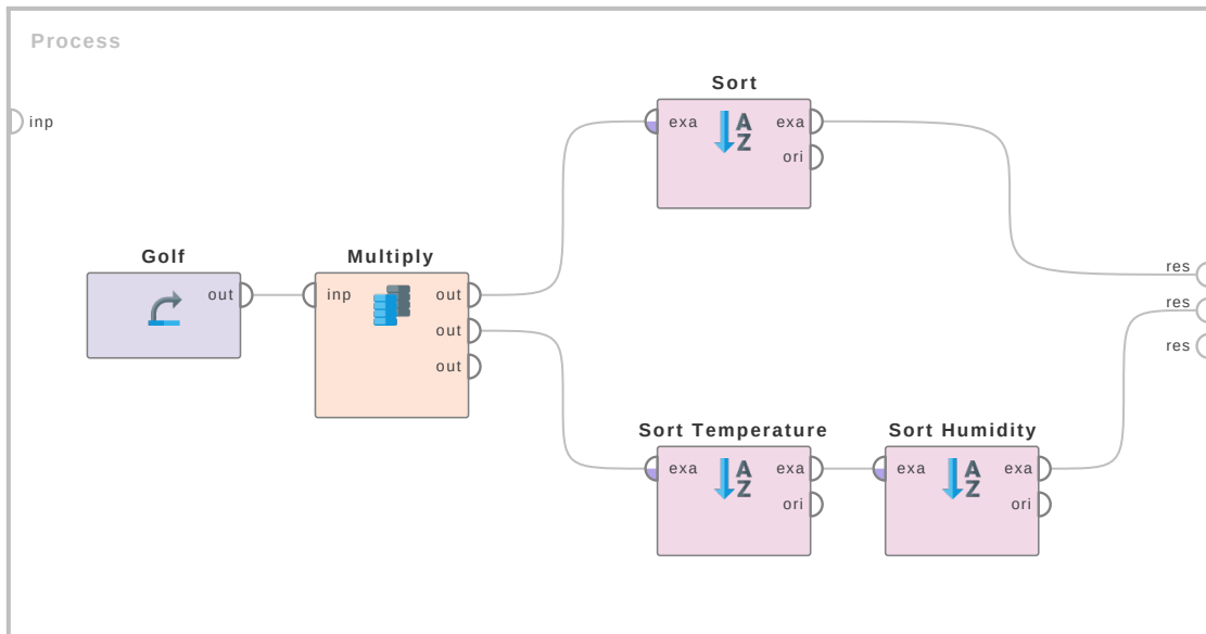
Figure 2.55: Tutorial process 'Sorting on multiple attributes'.
