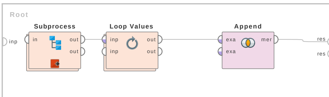
Figure 7.38: Tutorial process ‘The use of the Loop Values operator in complex preprocessing’.
