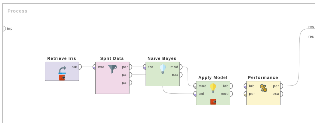
Figure 4.9: Tutorial process 'Apply Naive Bayes to the Iris Data Set'.
