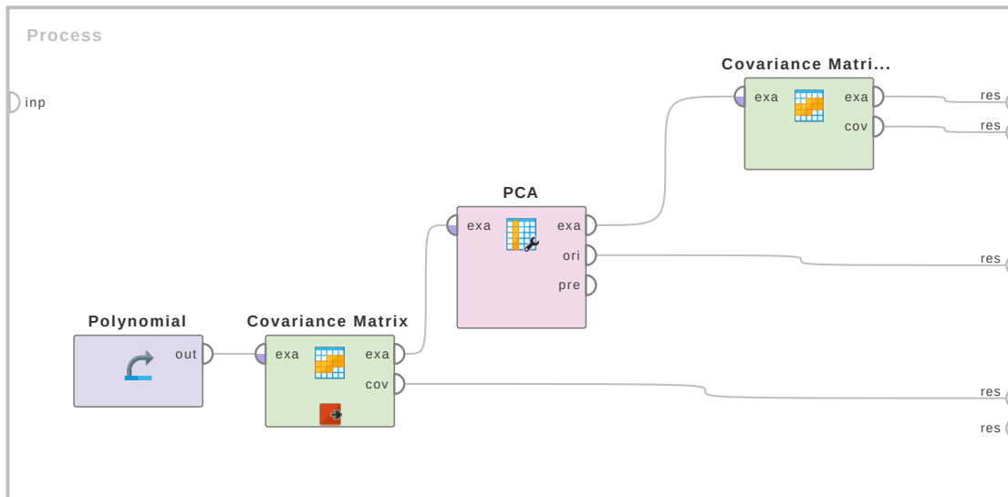
Figure 3.19: Tutorial process 'Dimensionality reduction of the Polynomial data set using the Principal Component Analysis operator'.
