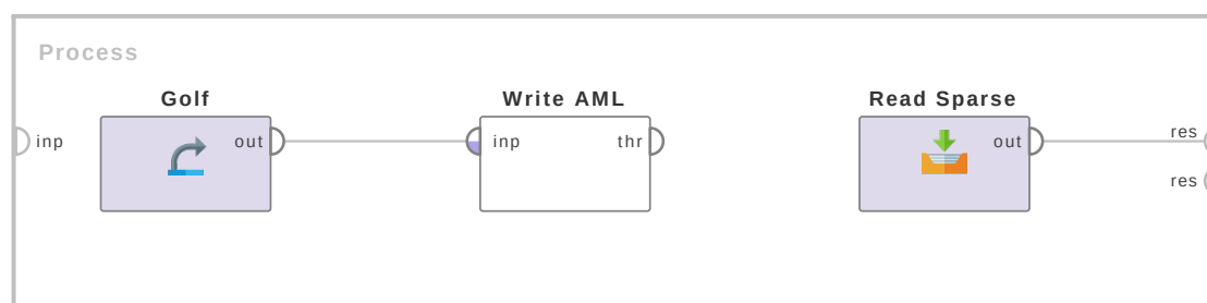
Figure 1.12: Tutorial process 'Writing and Reading a sparse file'.
