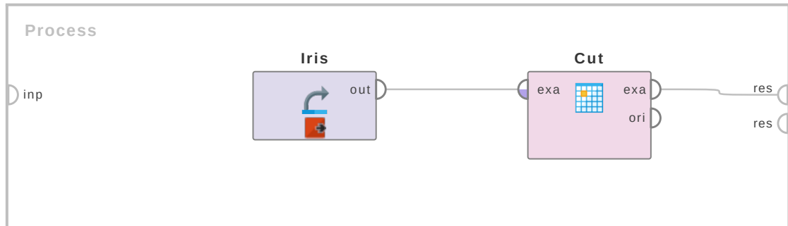
Figure 2.70: Tutorial process 'Applying the Cut operator on label of the Iris data set'.
