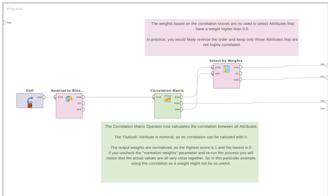
Figure 4.79: Tutorial process 'Correlation matrix of the Golf data set'.
