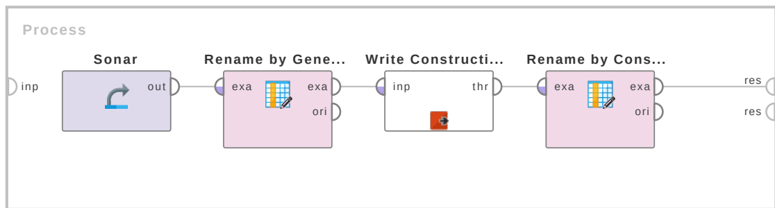
Figure 2.3: Tutorial process 'Renaming attributes by their construction descriptions'.
