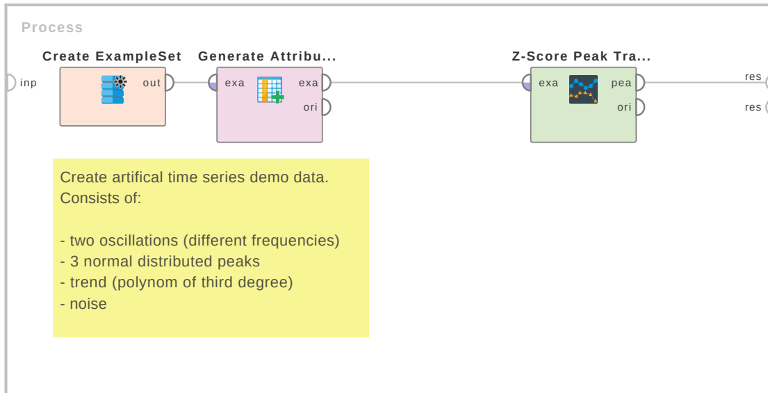
Figure 4.139: Tutorial process 'Detecting Peaks on artificial time series'.
