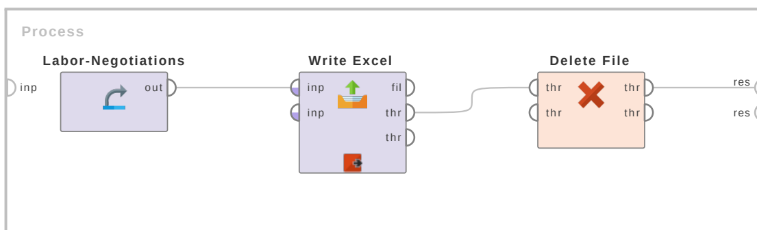
Figure 7.59: Tutorial process 'Writing the Labor-Negotiations data set into an Excel file and deleting it'.
