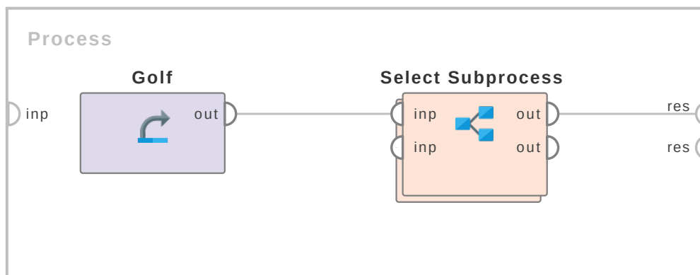
Figure 7.42: Tutorial process ‘Applying different classification operators on Golf data set using the Select Subprocess operator’.
