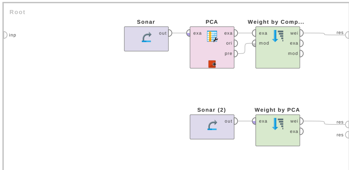
Figure 4.89: Tutorial process 'Calculating the attribute weights of the Sonar data set by PCA'.
