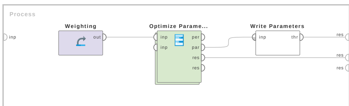
Figure 4.104: Tutorial process 'Finding optimal values of parameters of the SVM operator through the Optimize Parameters (Evolutionary) operator'.
