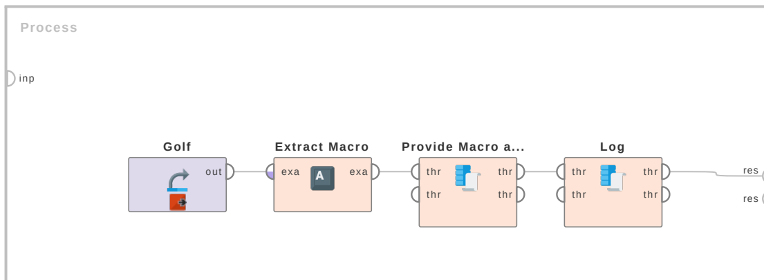
Figure 7.72: Tutorial process ‘Logging the value of a macro with or without the Provide Macro as Log Value operator’.
