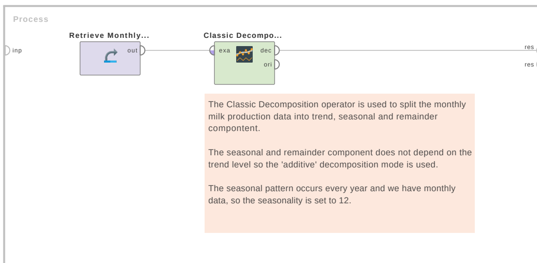
Figure 4.140: Tutorial process 'Classic Decomposition of the monthly milk production data set'.
