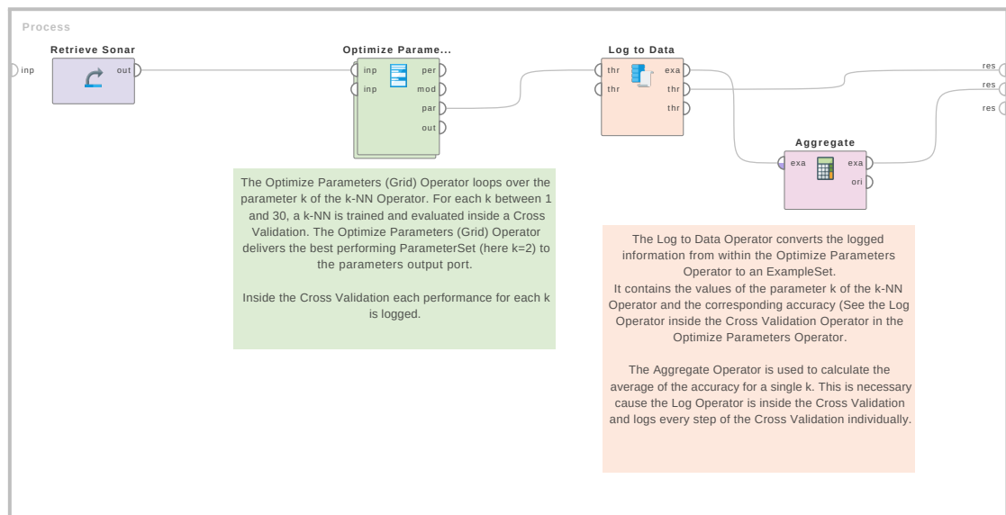
Figure 4.8: Tutorial process 'Optimizing k of a k-NN model and logging all results'.
