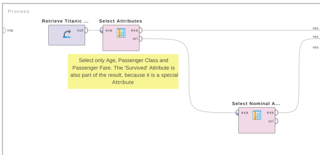
Figure 2.27: Tutorial process 'Selecting Attributes from the Titanic Data Sample'.
