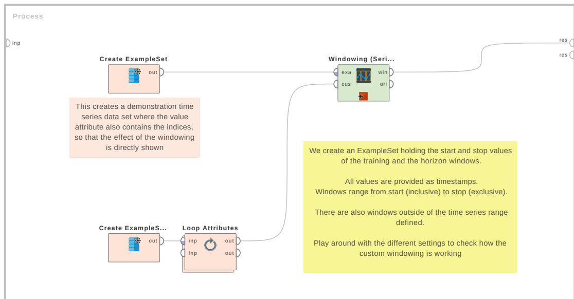
Figure 4.155: Tutorial process 'Custom Time Based Windowing of the Demo Data Set'.
