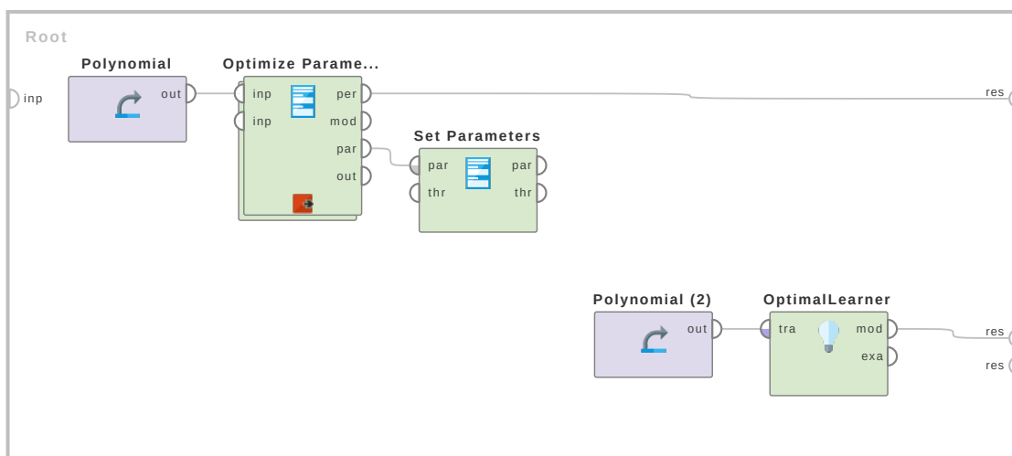
Figure 4.106: Tutorial process 'Building a model using an optimal parameter set'.
