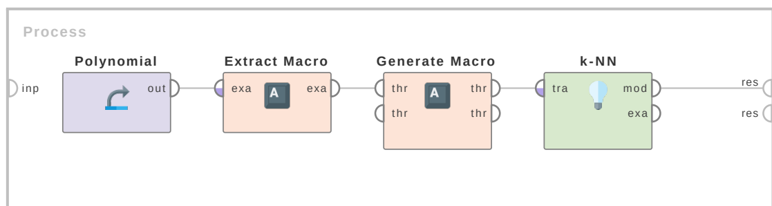
Figure 7.51: Tutorial process ‘Generating a new macro from an already existing macro’.
