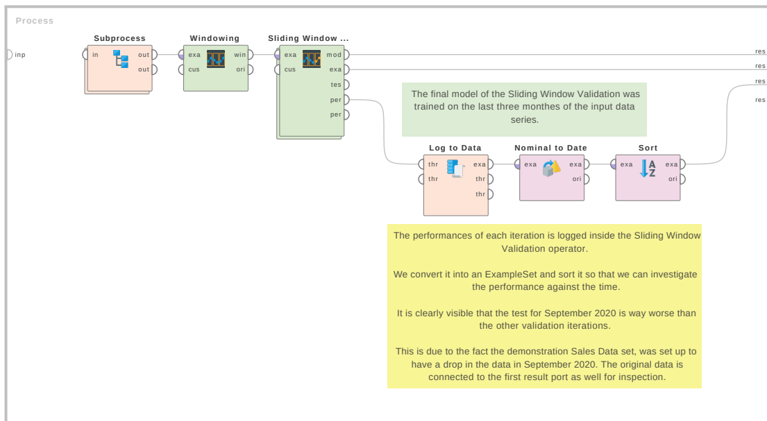
Figure 4.170: Tutorial process 'Use time based windowing to train and test on complete months of a daily Sales data set'.
