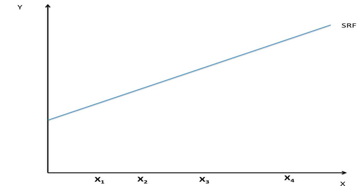
Figure 3.1: Least-Squares Criterion
