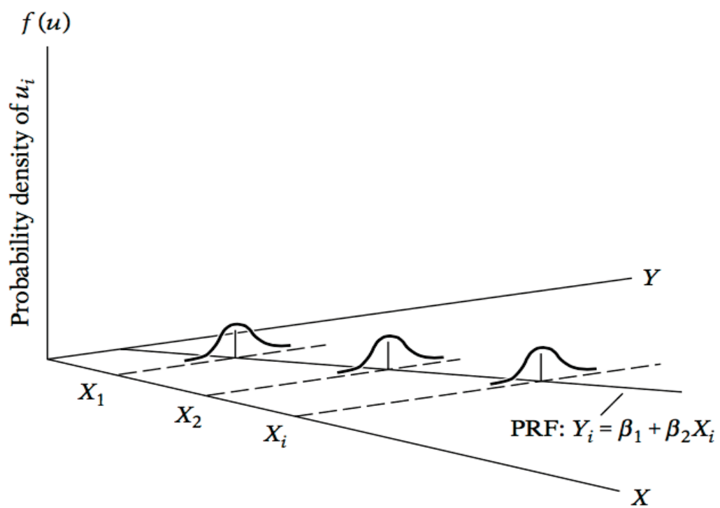
Figure 3.5: Homoscedasticity
