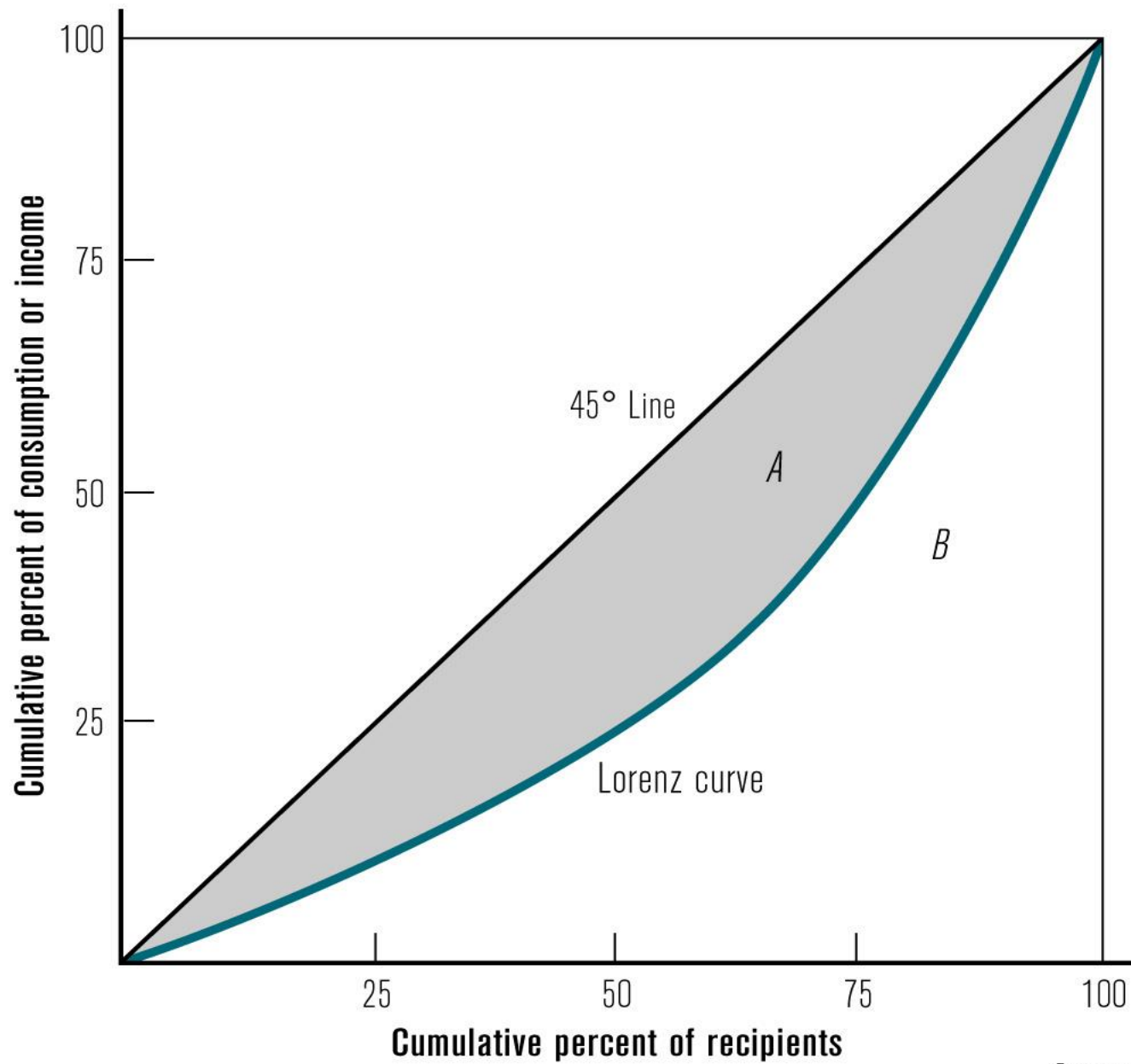
FIGURE 6.2 Lorenz Curve
