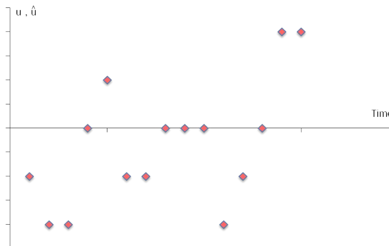
Figure 12-2: No autocorrelation among disturbance term
