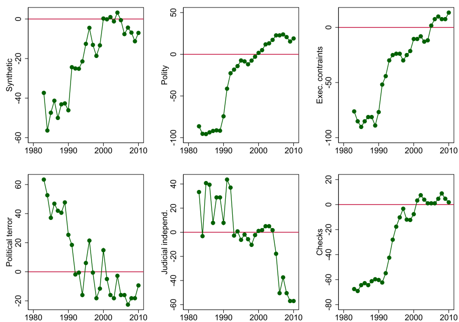
Fig. B1. Regional means for synthetic and sub-measures of institutions. Note: all measures are standardized, taking a mean of zero and standard deviation of one. Sources: see Appendix A .
