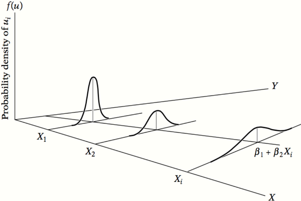
Figure 3.6: Heteroscedasticity
