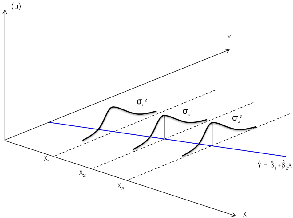
Figure 9.1: Homoscedasticity
