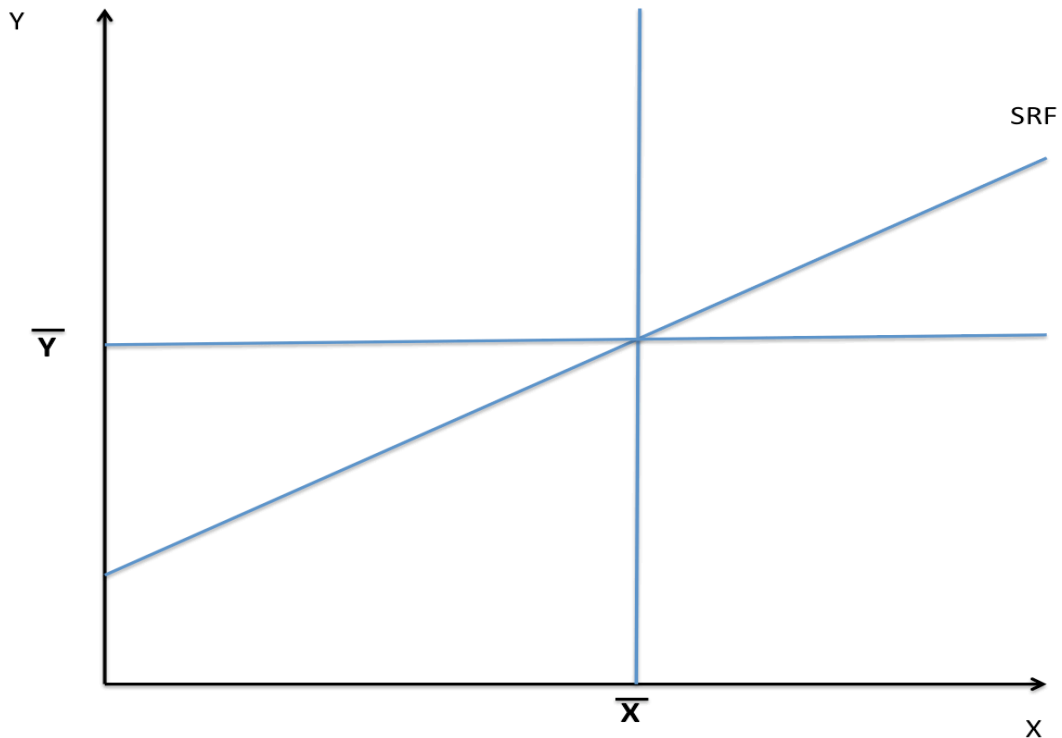
Figure 3.2: Sample Regression Line Based on the Data of Table 3.1
