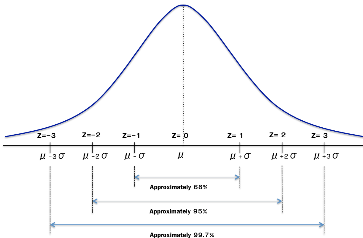
Figure 2-4: Normal Distribution
