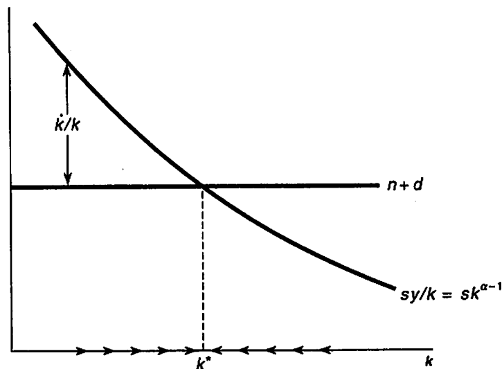
FIGURE 2.8 TRANSITION DYNAMICS
