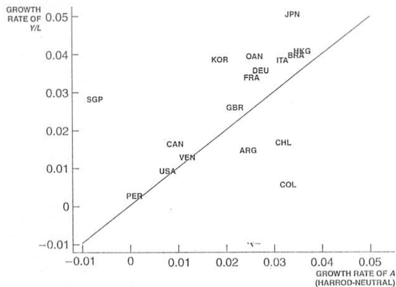
FIGURE 2.15 GROWTH ACCOUNTING
