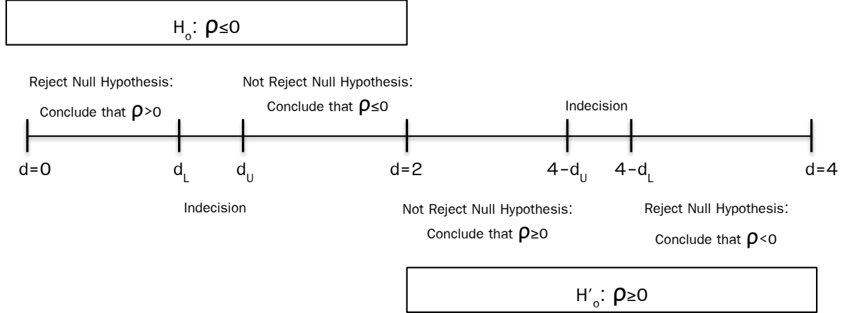
Figure 8-3: Criterion for rejecting or not rejecting the null hypothesis with DW-statistic
