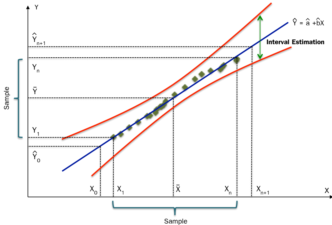
Figure 3-11: Interval Estimation
