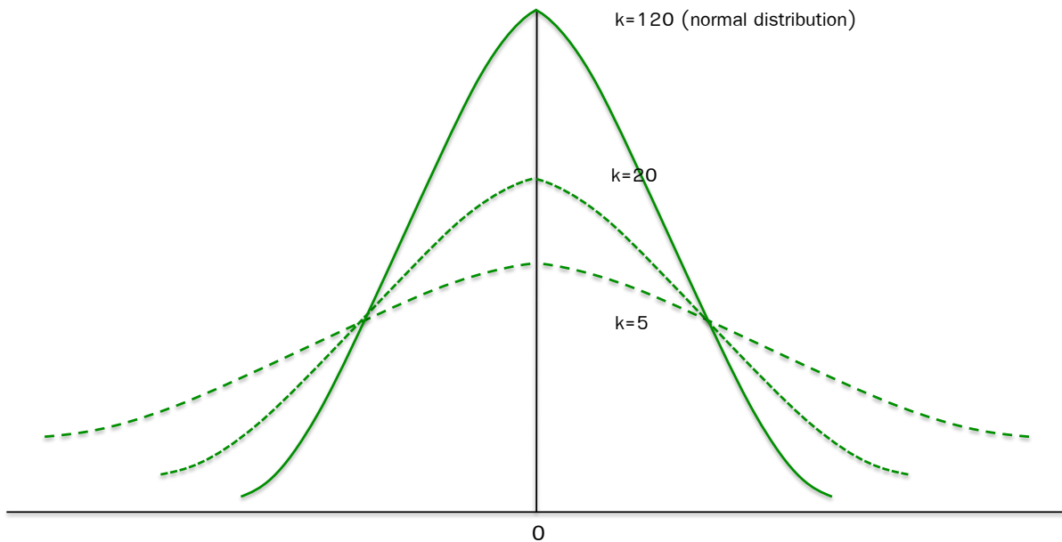
Figure 2-6: Student's t Distribution
