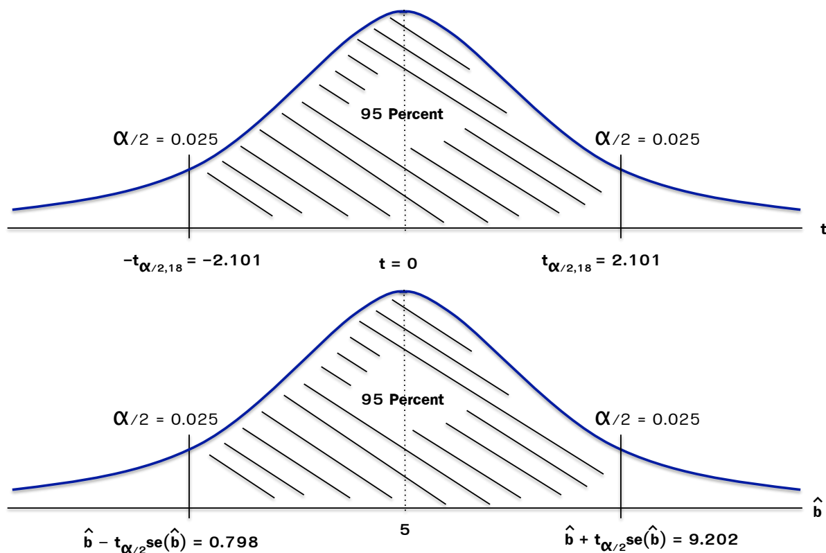
Figure 3-7: 95% Confidence Interval
