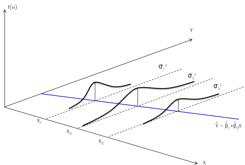
Figure 7-2: Heteroscedasticity
