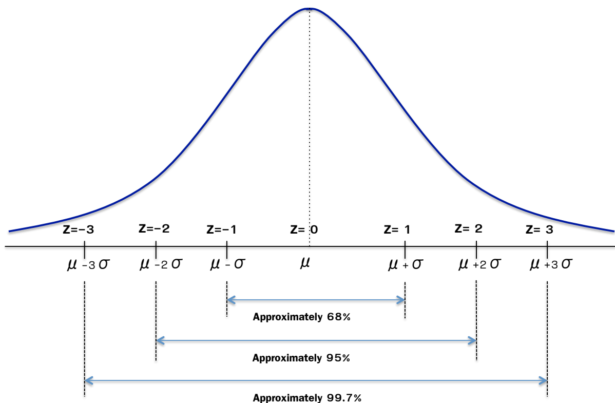
Figure 2-4: Normal Distribution
