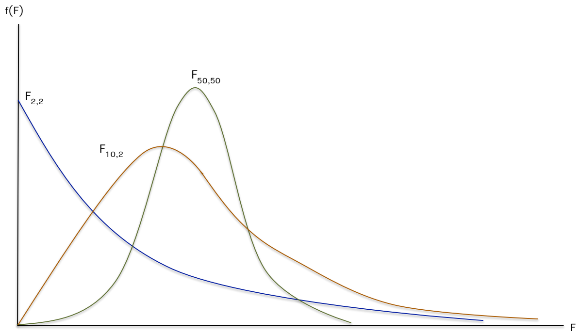
Figure 2-7: F Distribution
