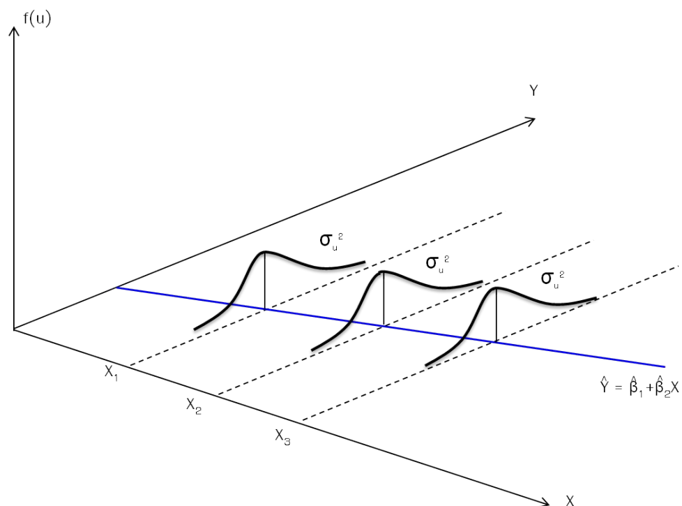
Figure 7-2: Heteroscedasticity
