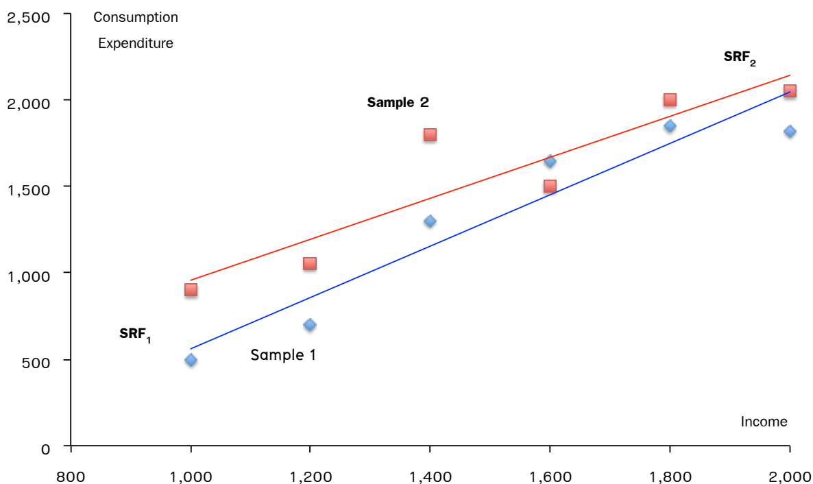
Figure 3-3: Scattergram for Each Group of Sample
