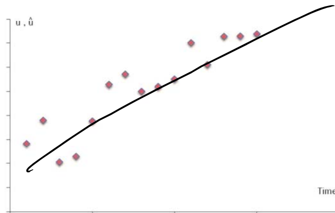
Figure 12-2: No autocorrelation among disturbance term
