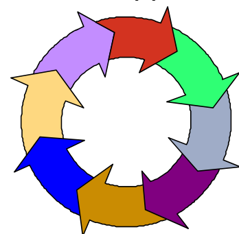
DMAIC Approach
