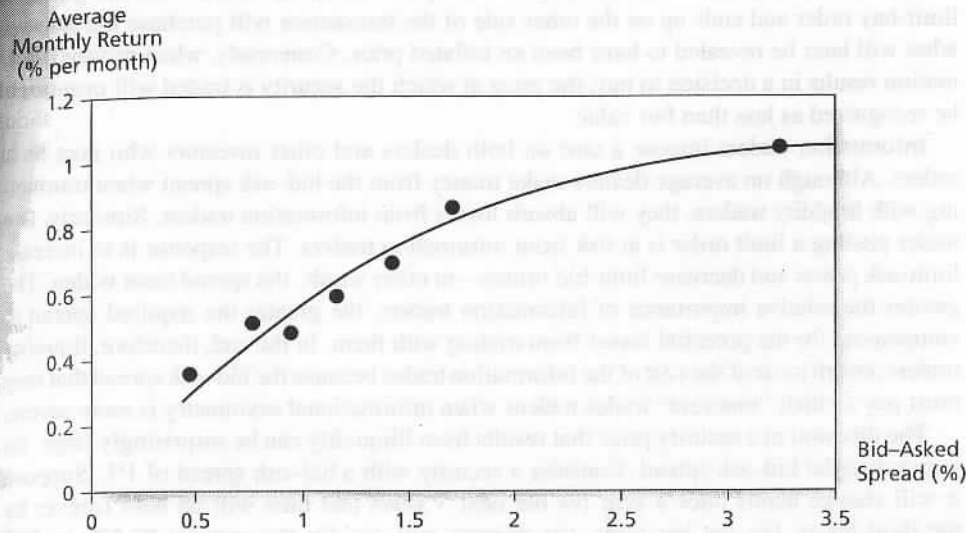
Figure 9.5 The relationship between illiquidity and average returns
