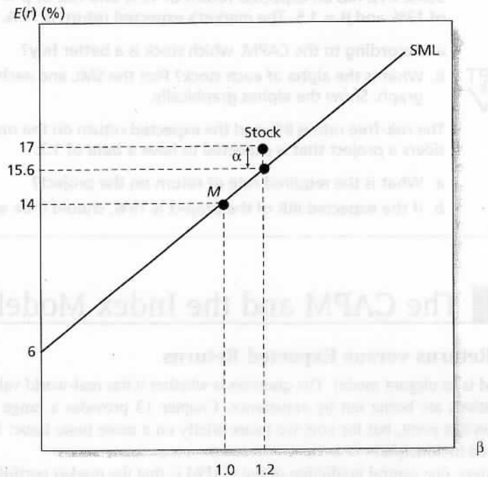
Figure 9.3 The SML and a positive-alpha stock
