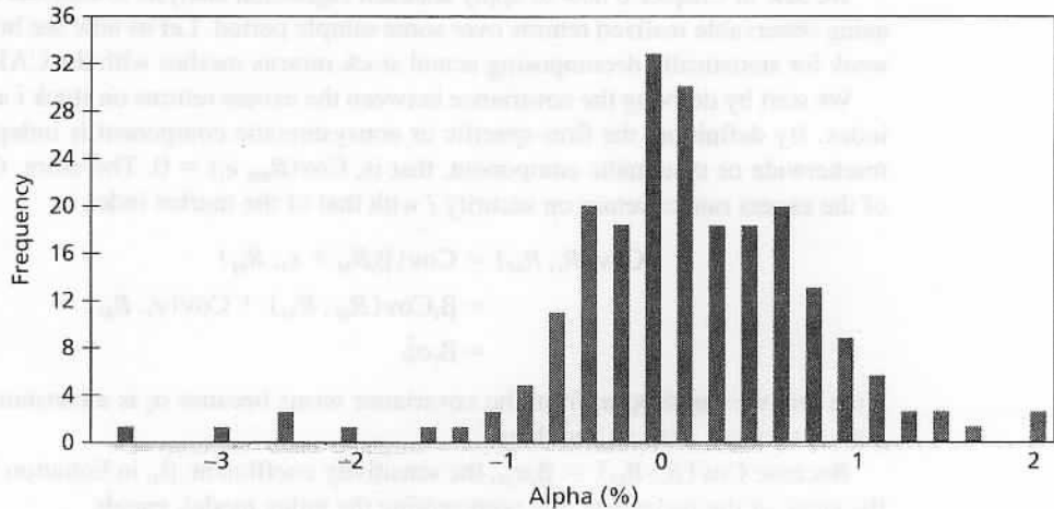
Figure 9.4 Estimates of individual mutual fund alphas, 1972–1991. This is a plot of the frequency distribution of estimated alphas for all-equity mutual funds with 10-year continuous records.
