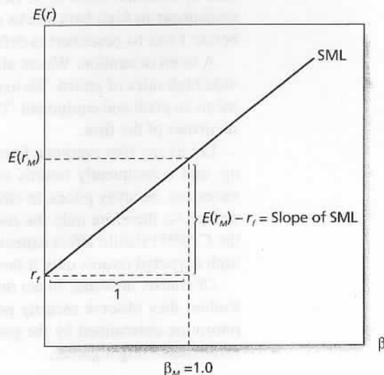
Figure 9.2 The security market line
