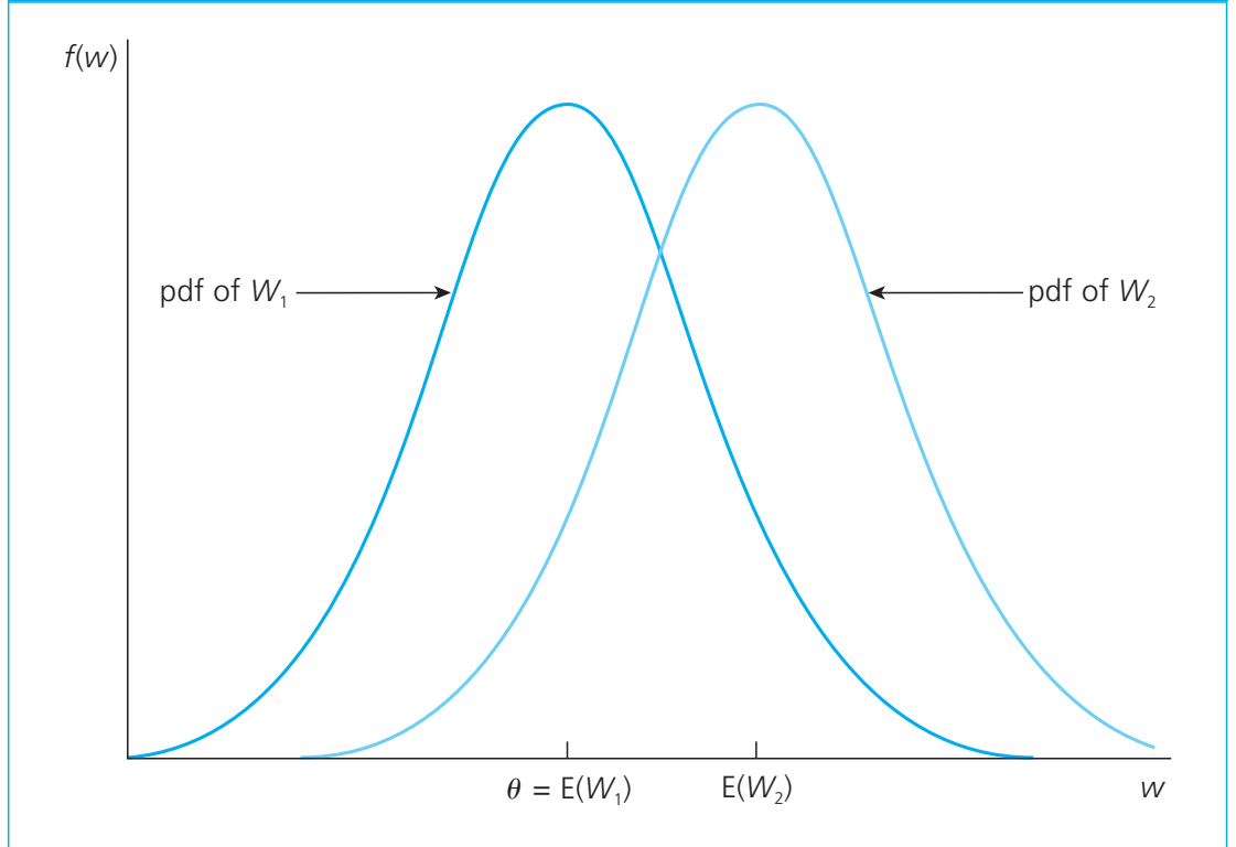
FIGURE C.1 An unbiased estimator, W_1 , and an estimator with positive bias, W_2 .
