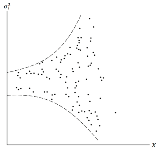
Figure 11.6 : Error variance proportional to X^2
