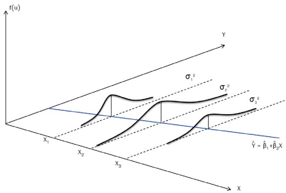
Figure 11.2: Heteroscedasticity
