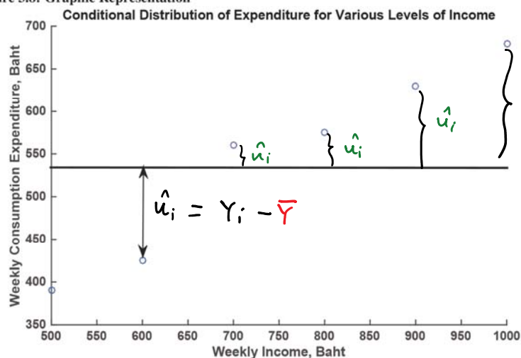
Figure 3.8: Graphic Representation
