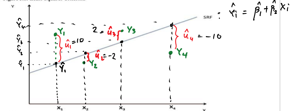
Figure 3.1: Least-Squares Criterion
