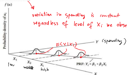
Figure 3.5: Homoscedasticity
